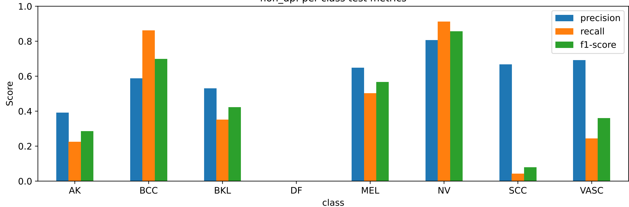
non_dp: per-class test metrics
