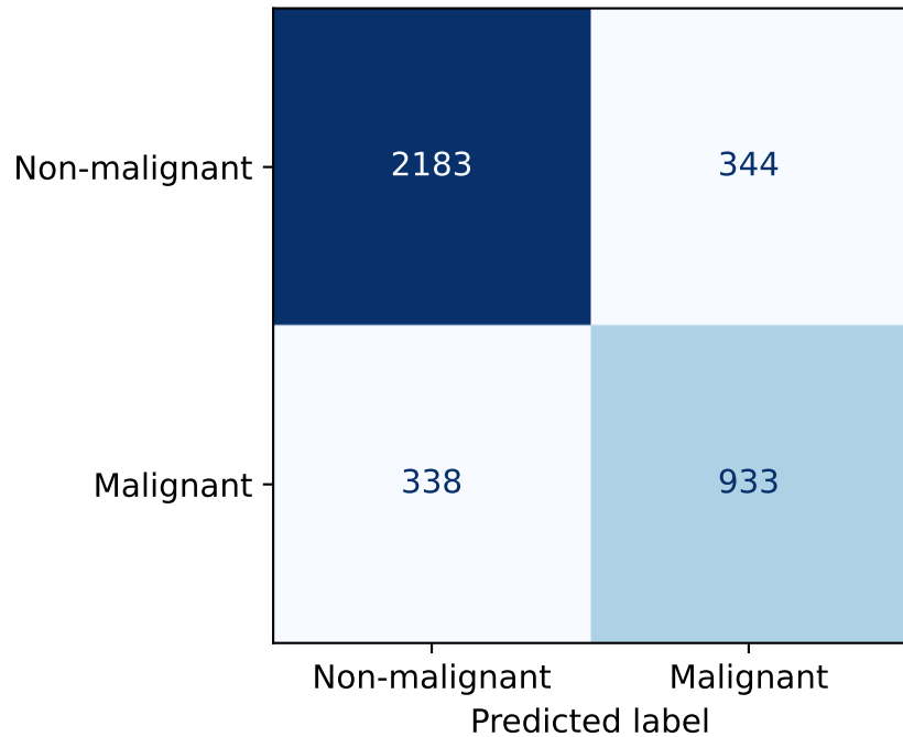
non_dp: Default threshold 0.5
