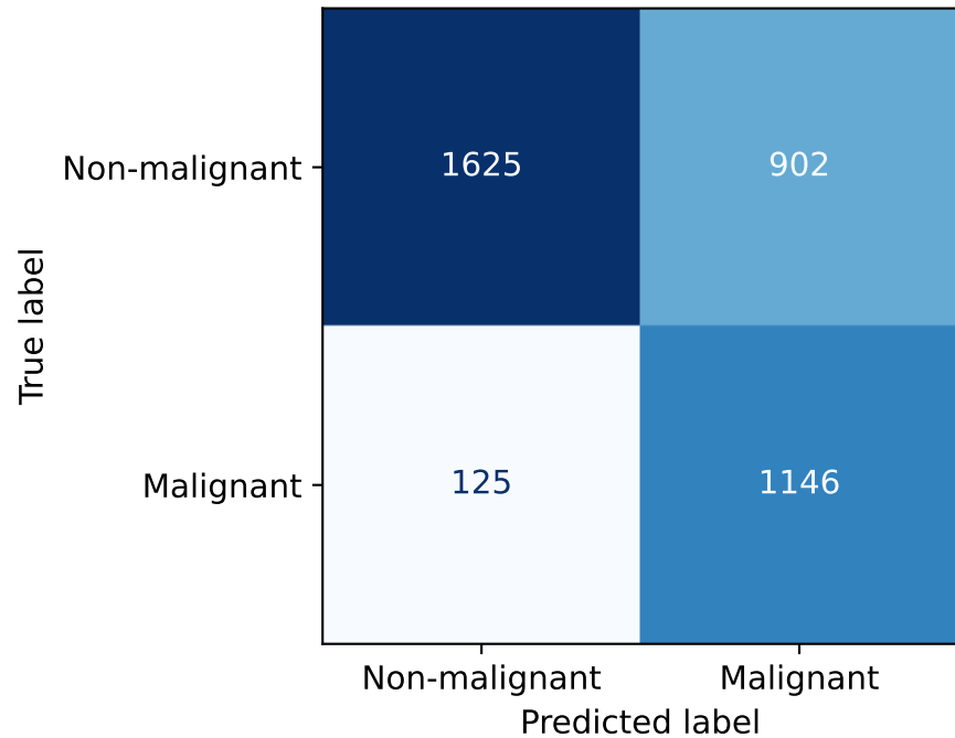
non_dp: Validation-selected threshold
