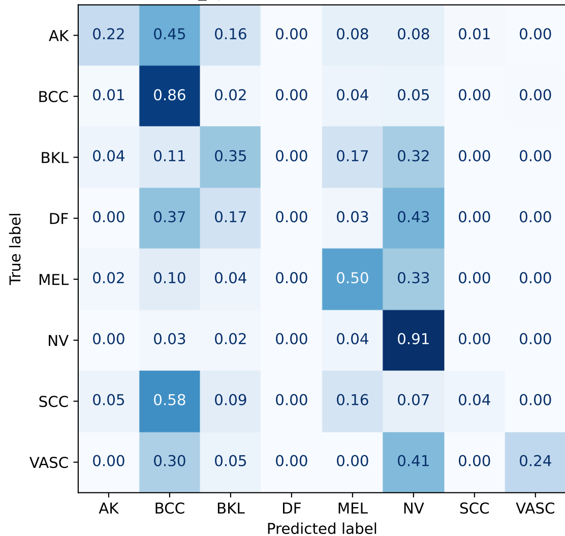
non_dp: multiclass — Row-normalized
