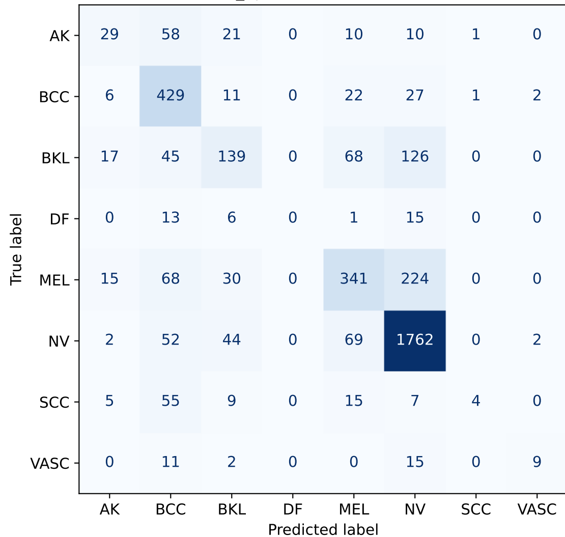
non_dp: multiclass — Counts
