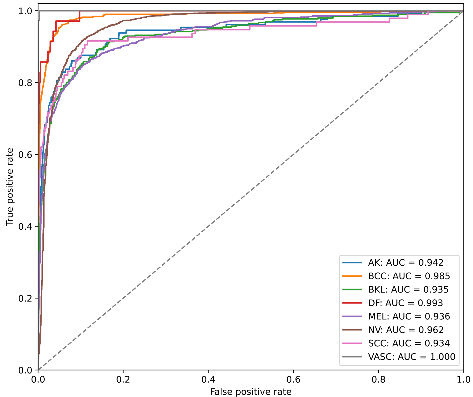
Multiclass test ROC — one-vs-rest
