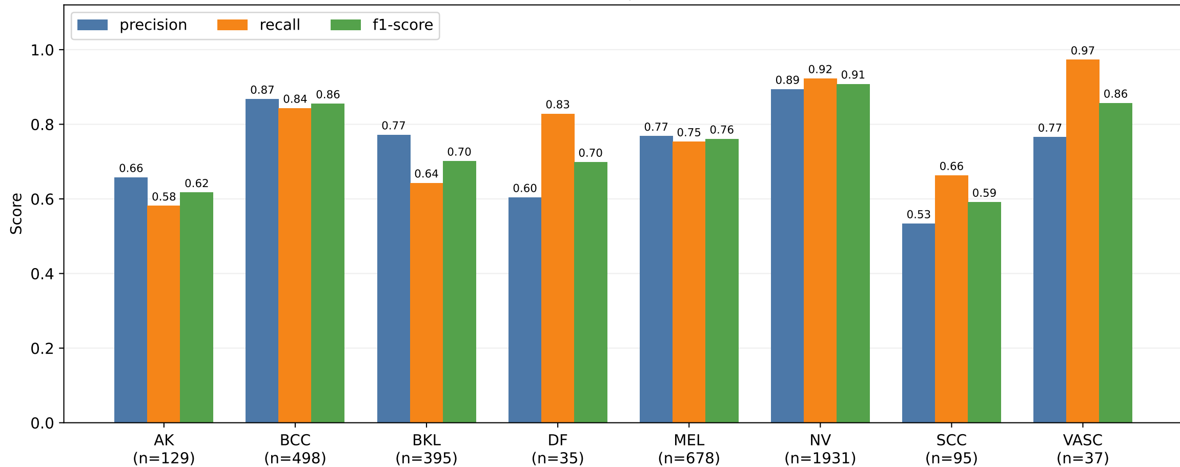
Per-class test performance
