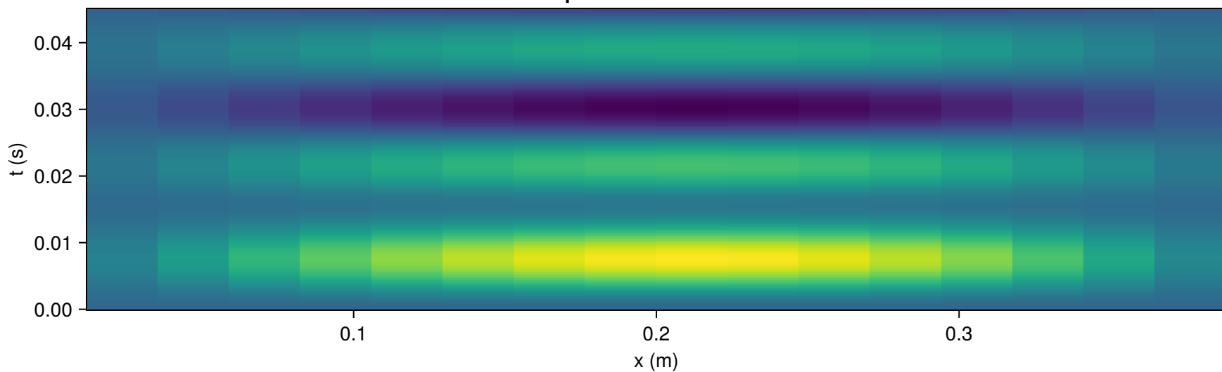
Interpolation – Prediction
