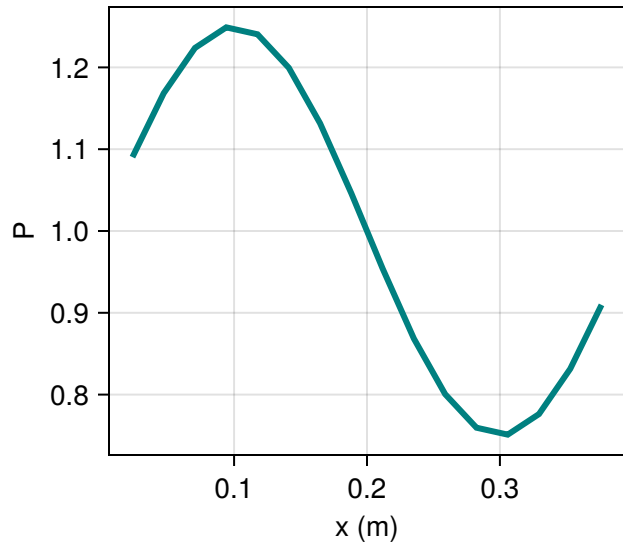
Ground Truth Modulus P_0(x)
