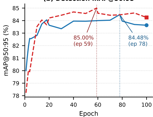
(b) Detection mAP@50:95
