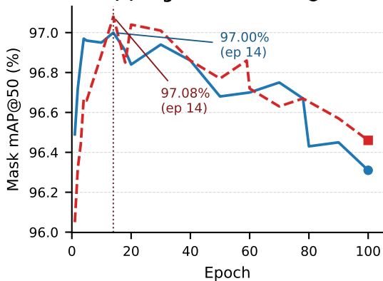
(c) Segmentation mAP@50
