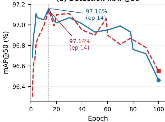
(a) Detection mAP@50
