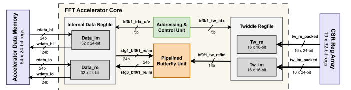
Fig. 2: FFT accelerator core architecture, showing the register file, 2\times pipelined butterfly unit, twiddle CSR interface, and wide paired memory port.
