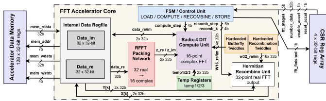
Fig. 6: RFFT-based accelerator core architecture with memory access - 16-point FFT using two Radix-4 stages. This includes real to complex packing, hardcoded twiddle factors, and a Hermitian recombination unit.
