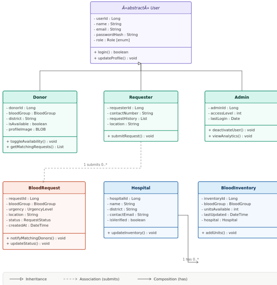
Figure 3-2: Class Diagram
