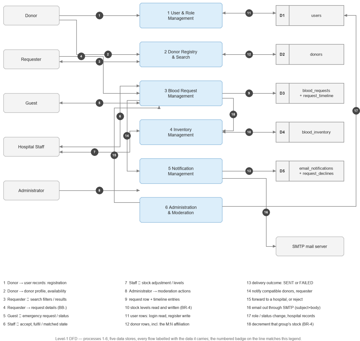
Figure 3-5: Level-1 Data Flow Diagram
