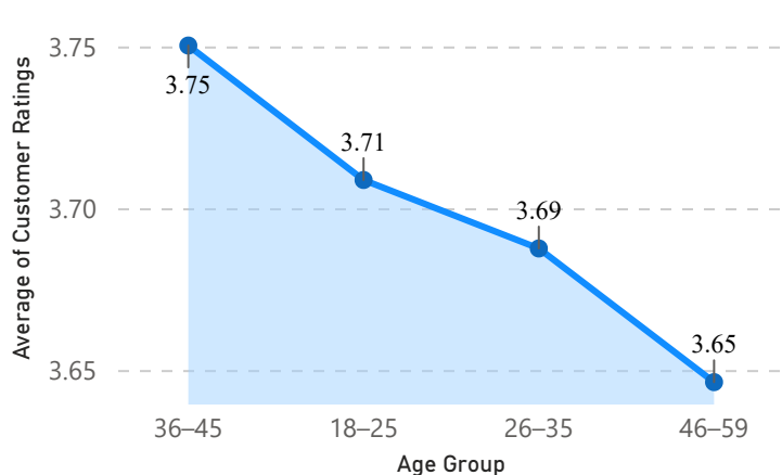
Average of Customer Ratings by Age Group
