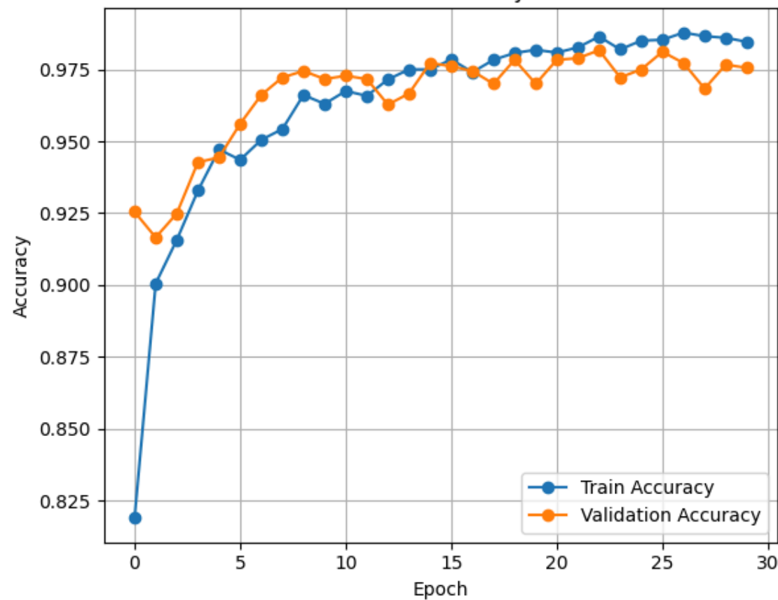
Model Accuracy
