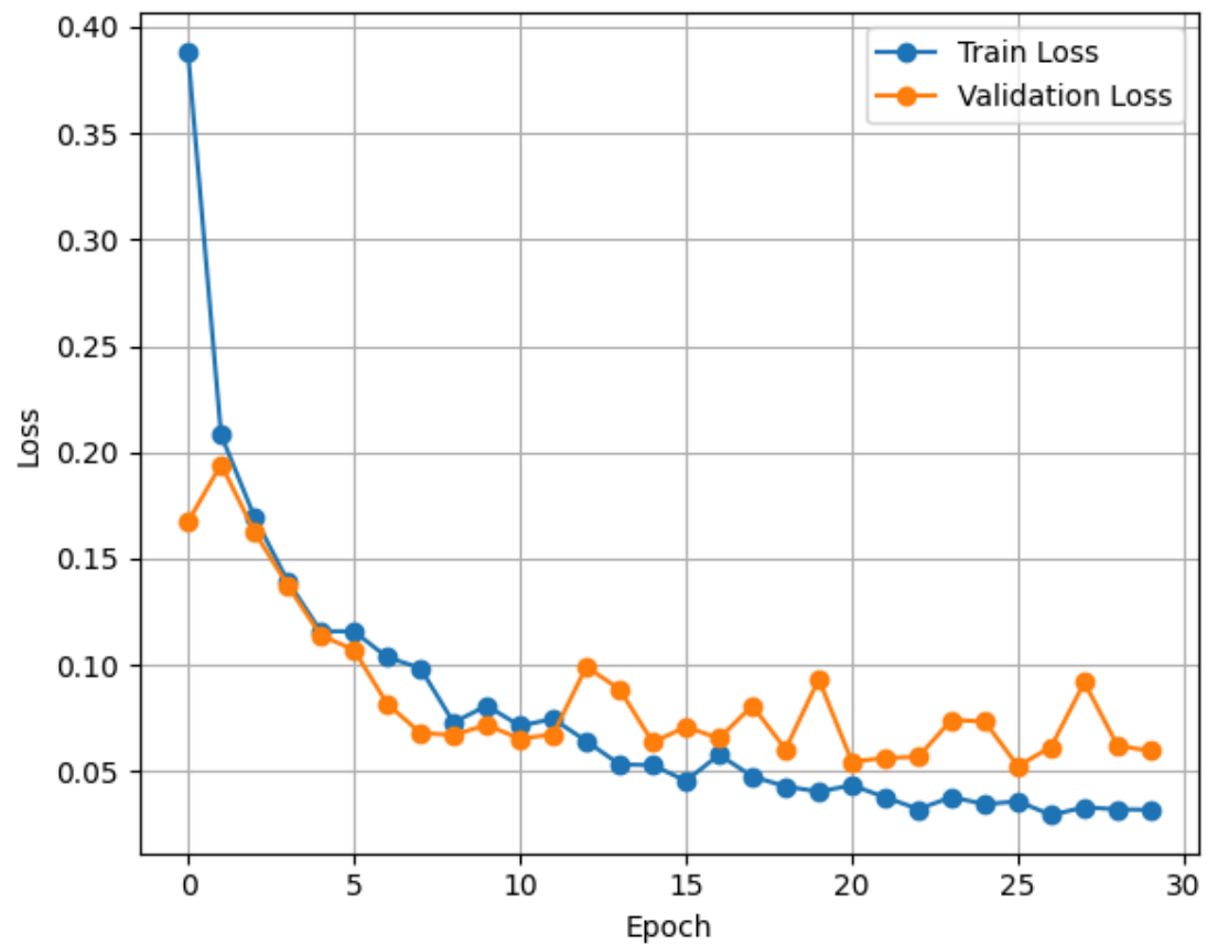
Model Loss
