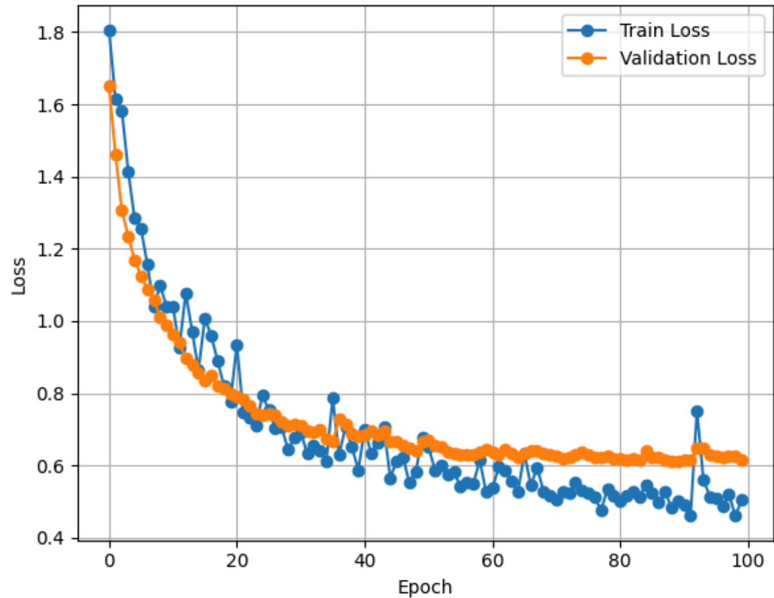
Model Loss
