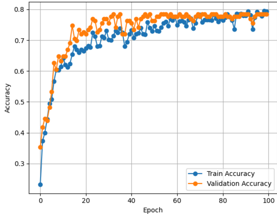
Model Accuracy
