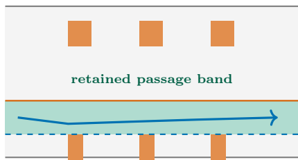
Group-level MIKU bounds
