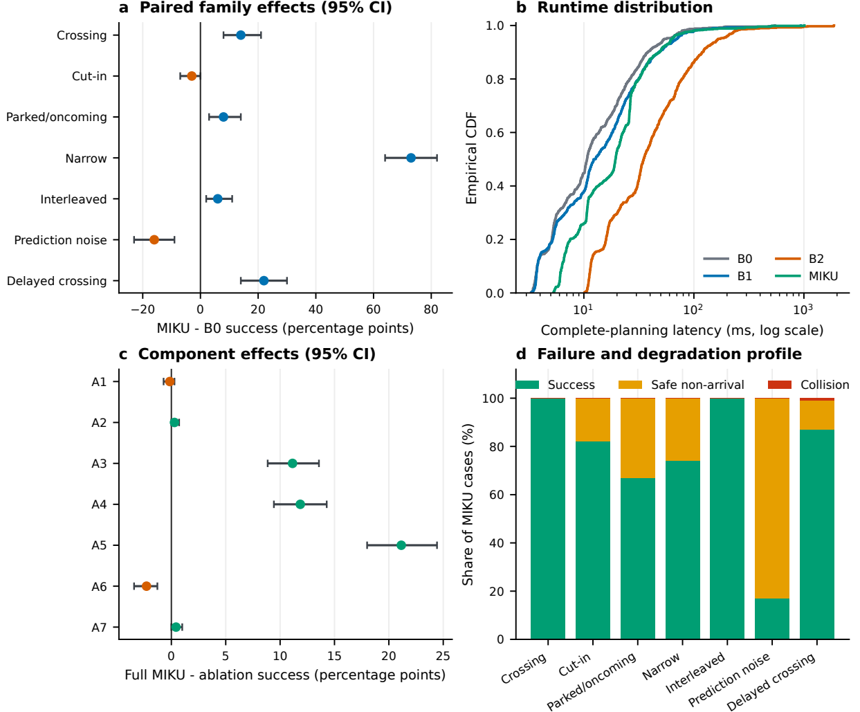
Fig. 2. CSV-generated evidence dashboard. (a) Paired MIKU–B0 success-rate effects by family with 95% CIs. (b) Empirical CDF of complete-planning latency. (c) Full-MIKU success-rate effects relative to each ablation. (d) MIKU success, safe non-arrival, and collision outcomes by family.
