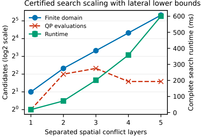
Fig. 4. Finite-domain stress diagnostic with two feasible bands per separated spatial layer and one dynamic crossing. The squared distance of each corridor to l = 0 supplies an admissible lower bound; the domain/evaluation gap exposes actual pruning.
