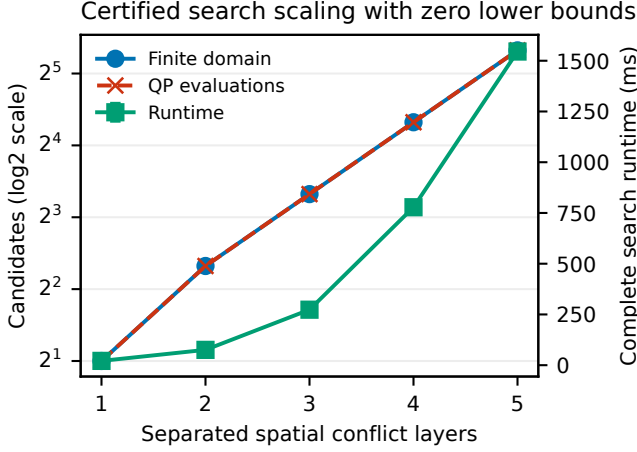
Fig. 4. Finite-domain stress diagnostic with two feasible bands per separated spatial layer and one dynamic crossing. Domain size equals QP evaluations because the present zero lower bound gives no pruning.
