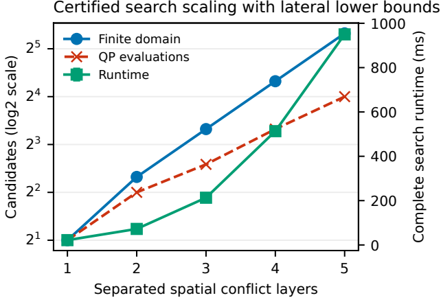
Fig. 5. Finite-domain stress diagnostic with two feasible bands per separated spatial layer and one dynamic crossing. The solved path-QP value supplies an admissible branch lower bound; the domain/evaluation gap exposes actual pruning.
