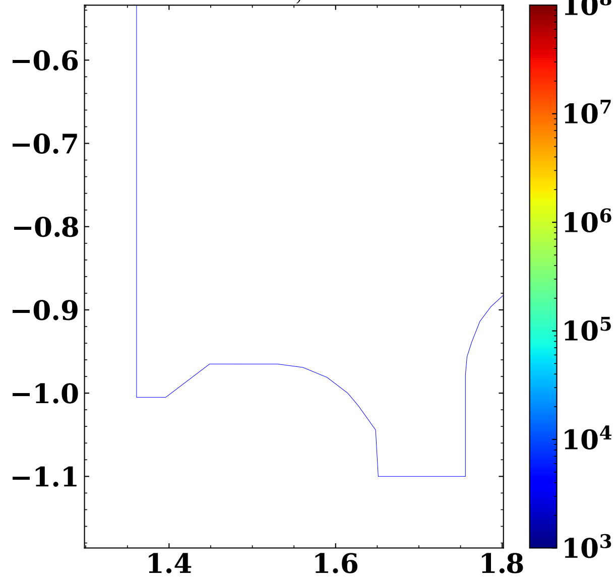
3.2e19 S_{E,Rec}^{D^1} (Wm -3 )
