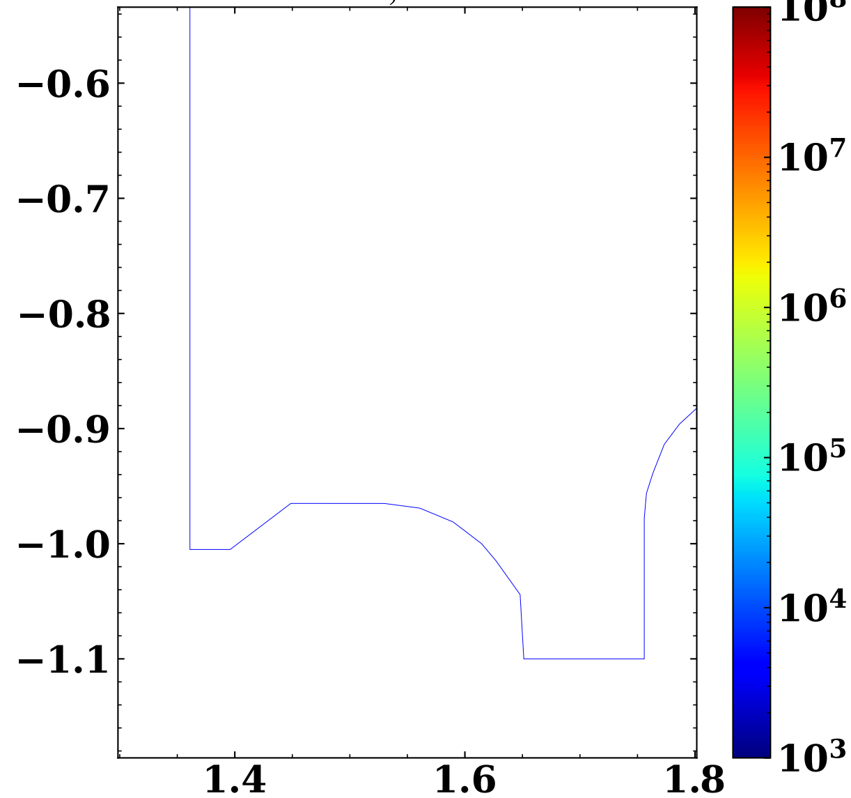
5e19 S_{E,Rec}^{D^1} (Wm -3 )
