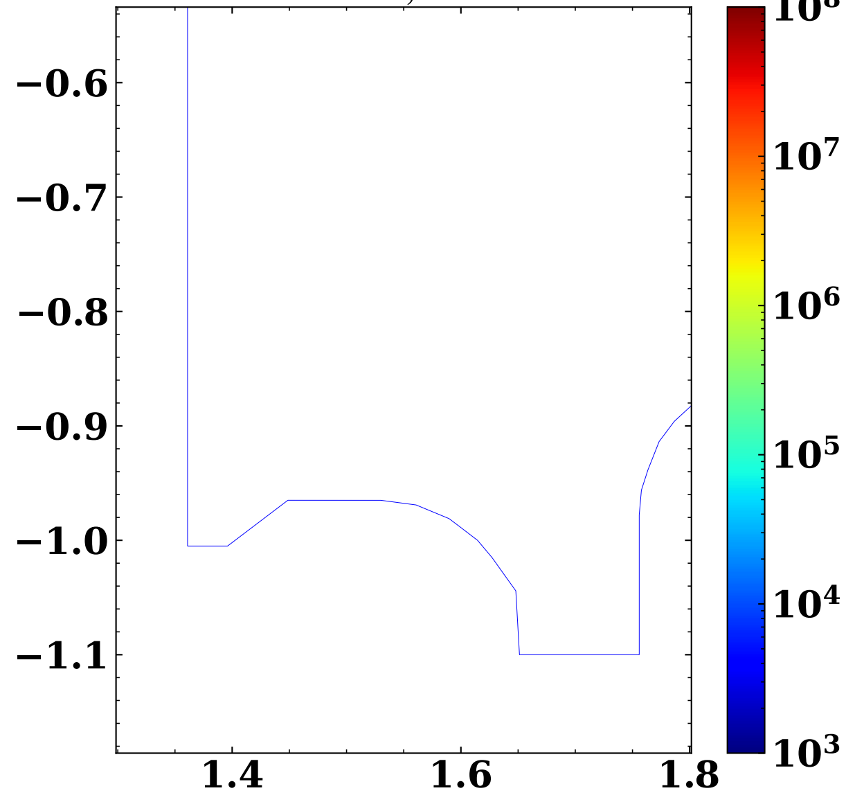
4.6e19 S_{E,Rec}^{D^1} (Wm -3 )
