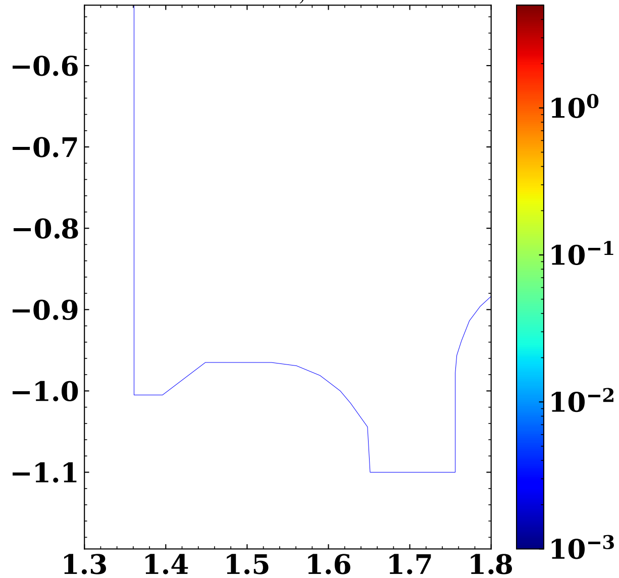
5.8e19 S_{M,CX}^{D^0}(\text{Nm}^{-3})
