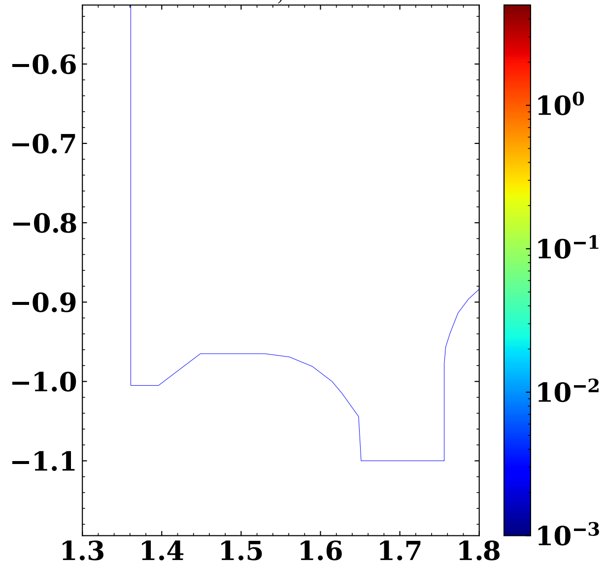
4e19 S_{M,CX}^{D^0}(\text{Nm}^{-3})
