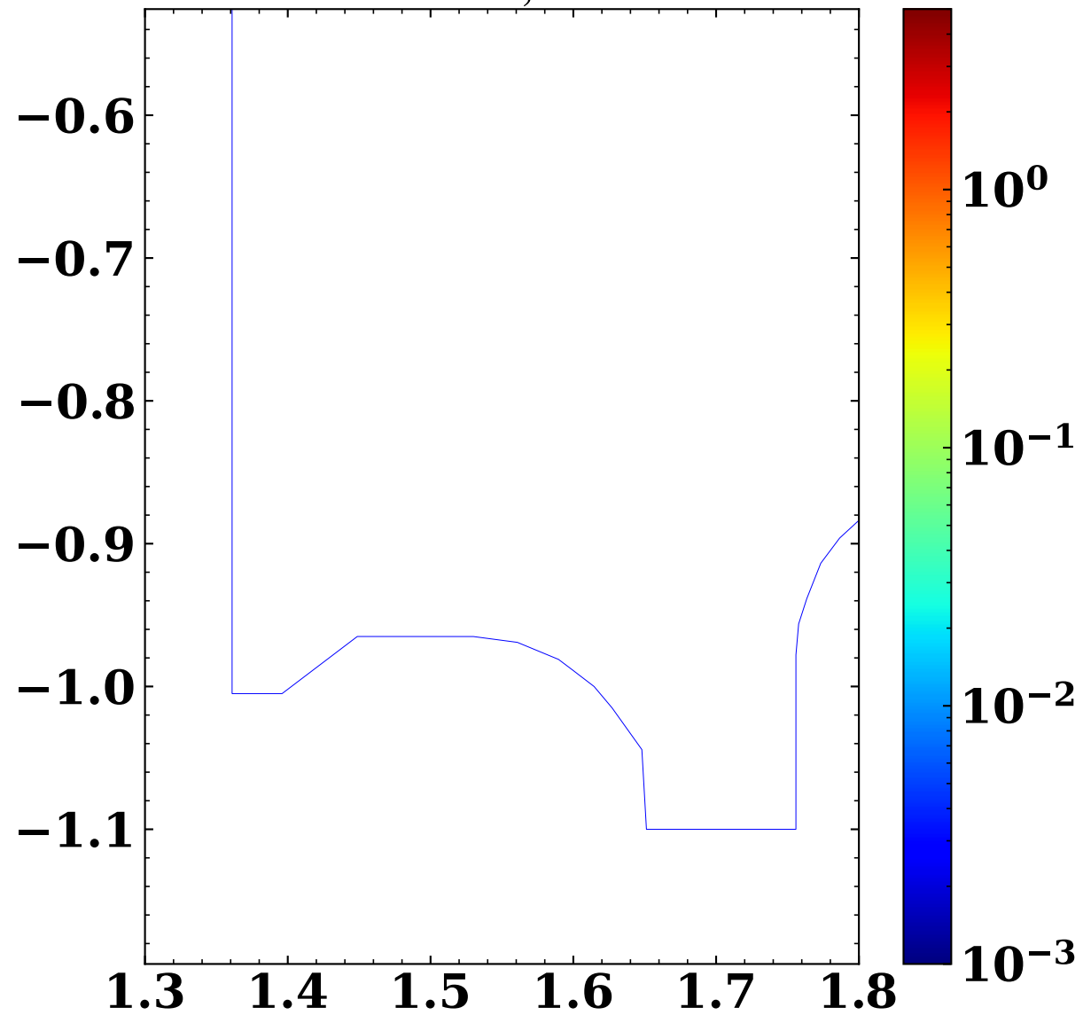
4.6e19 S_{M,CX}^{D^0}(\text{Nm}^{-3})
