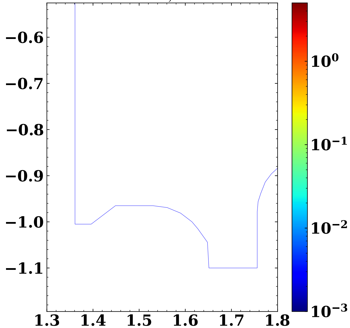
3.2e19 S_{M,CX}^{D^0}(\text{Nm}^{-3})
