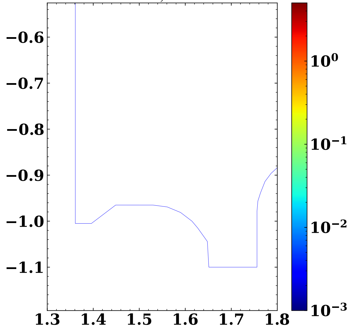
5e19 S_{M,CX}^{D^0}(\text{Nm}^{-3})
