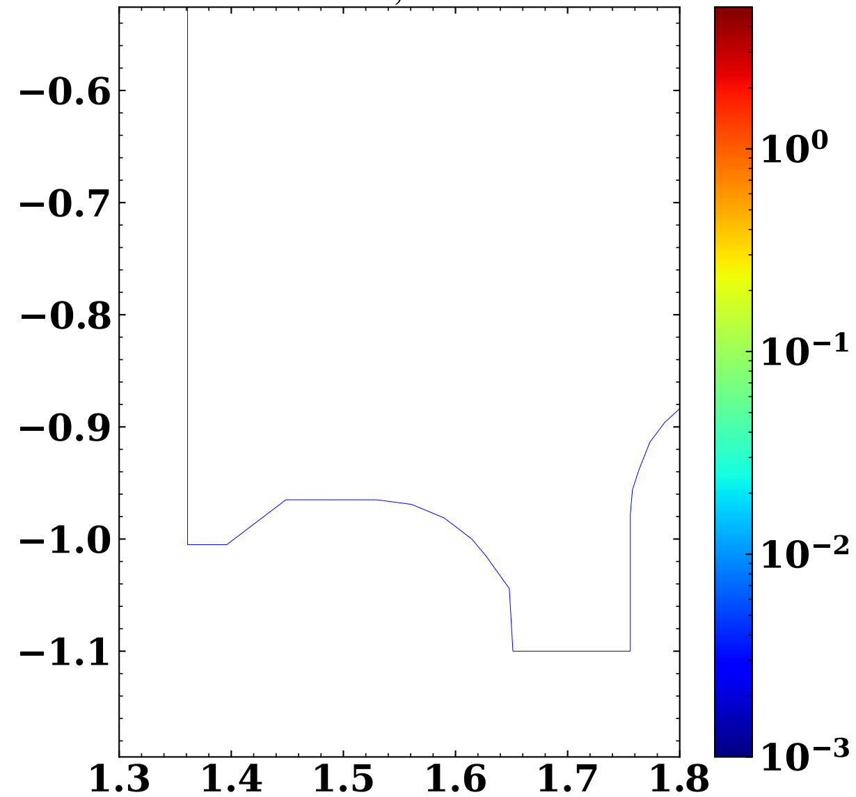
4e19 S_{M,CX}^{D^0}(\text{Nm}^{-3})
