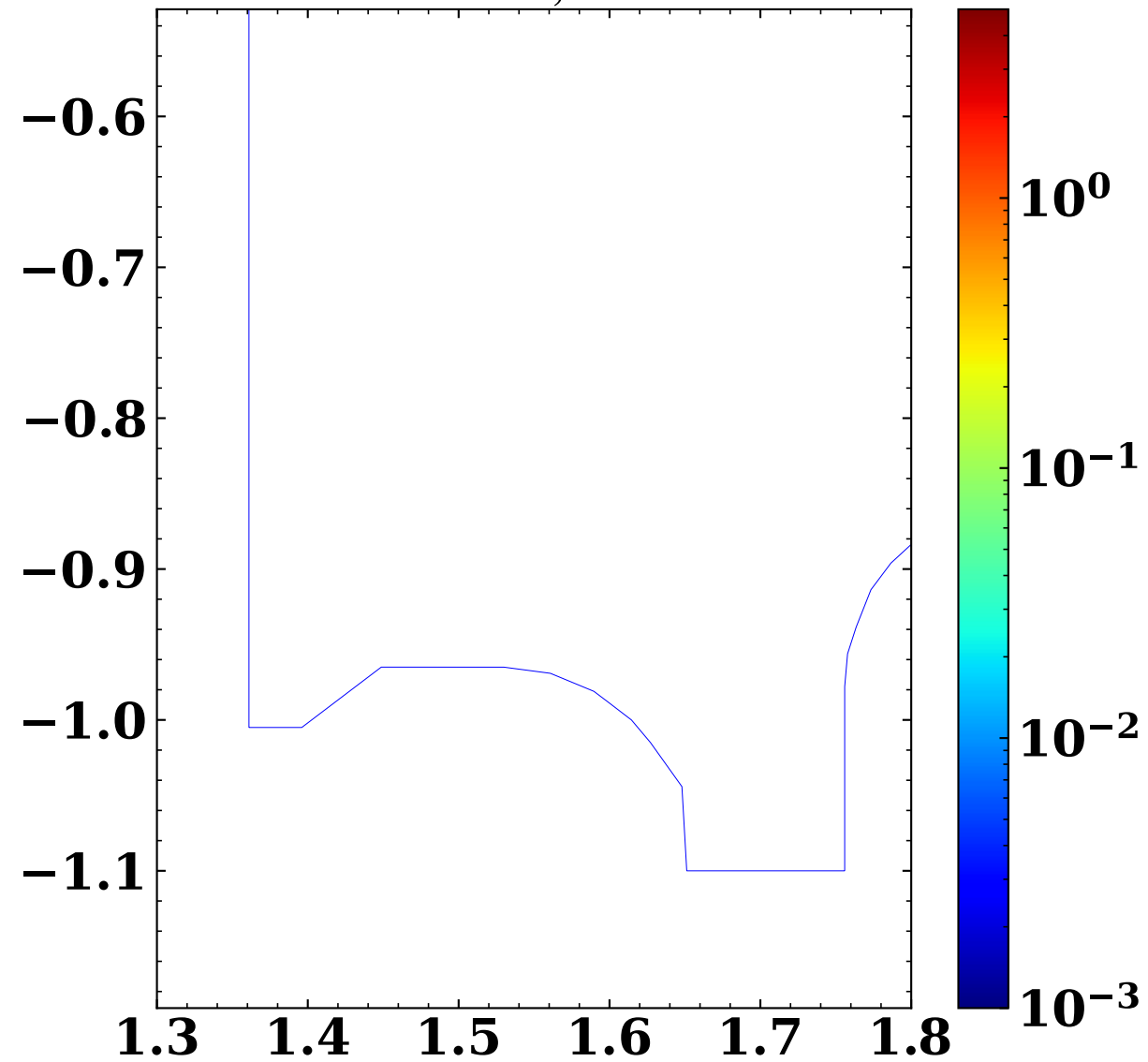
3.2e19 S_{M,Ela}^{D_2^0} (Nm -3 )
