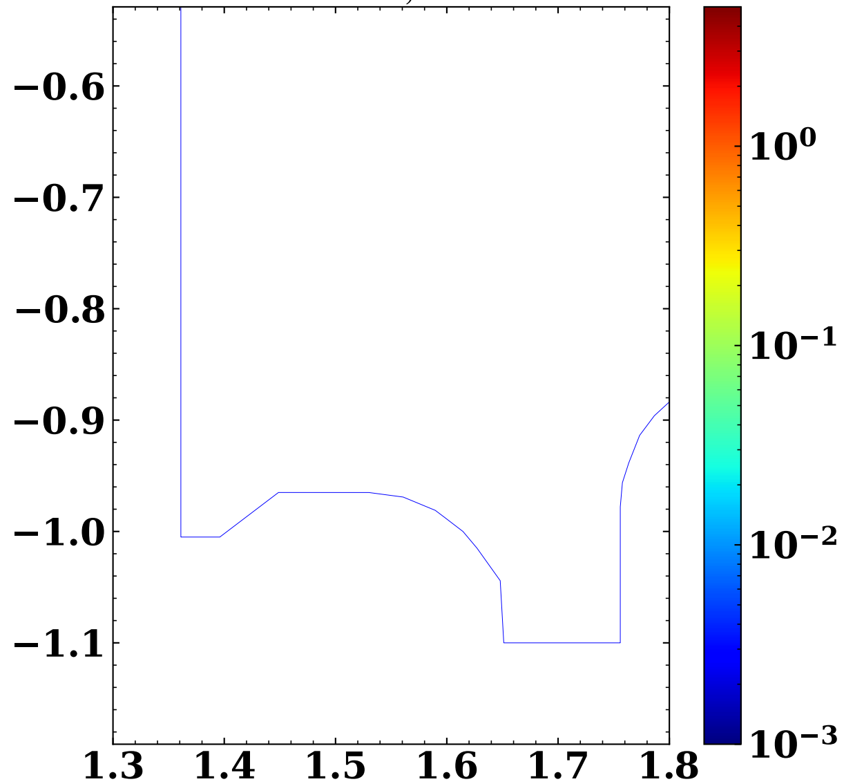
4.6e19 S_{M,Ela}^{D_2^0} (Nm -3 )
