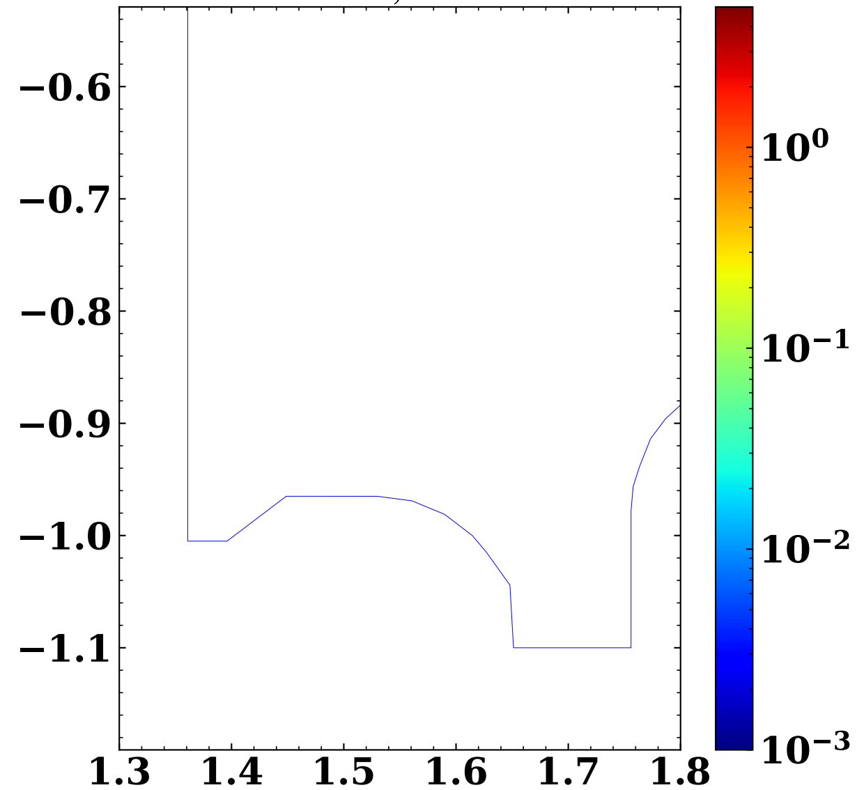
4e19 S_{M,Ela}^{D_2^0} (Nm -3 )
