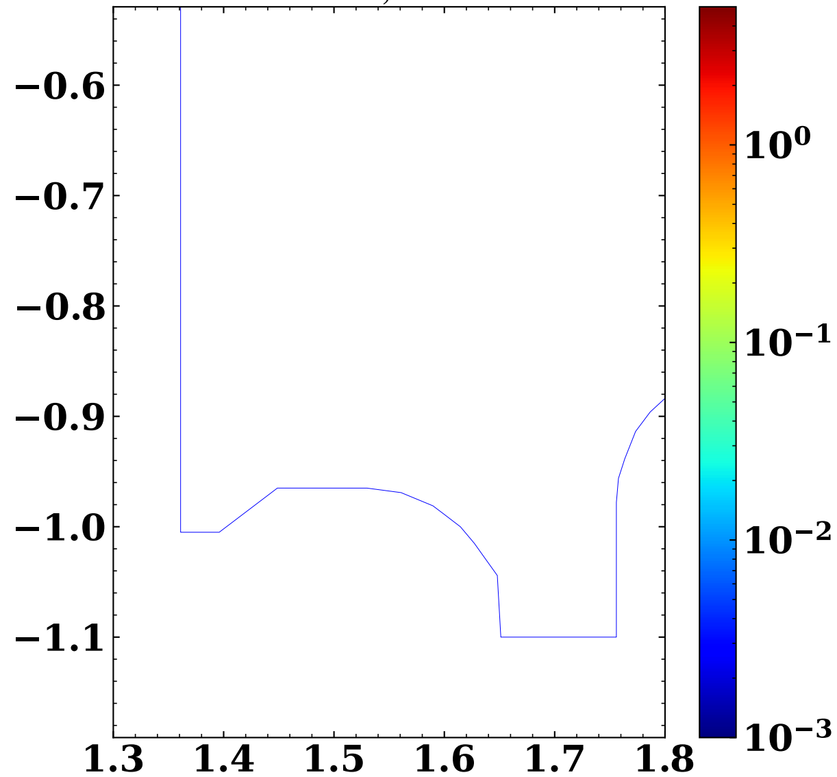
5e19 S_{M,Ela}^{D_2^0} (Nm -3 )
