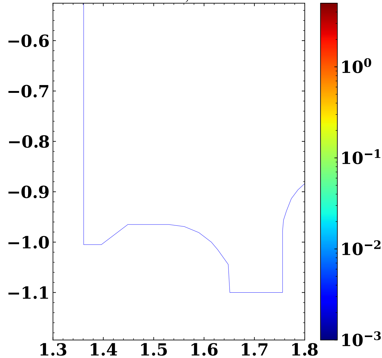
3.6e19 S_{M,Ion}^{D^0} (Nm -3 )
