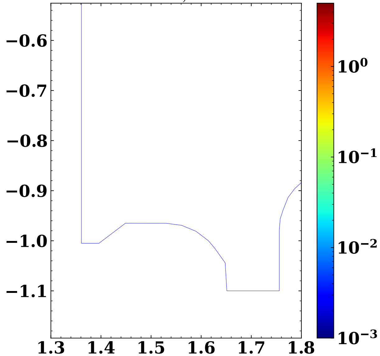
4.6e19 S_{M,Ion}^{D^0} (Nm -3 )
