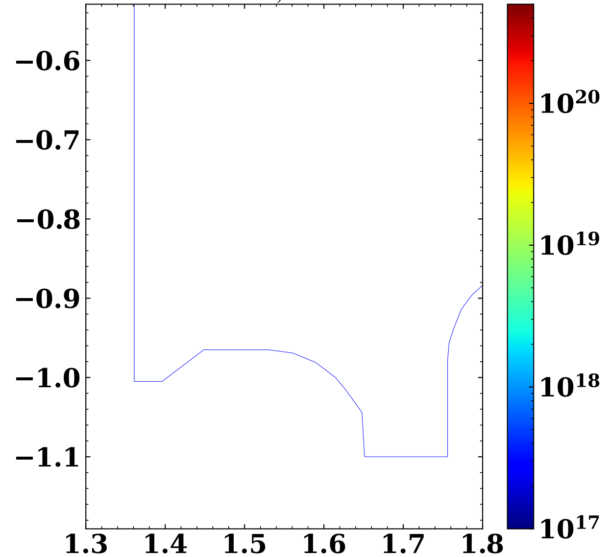
5.8e19 S_{n,DS4}^{D_2^+} (\text{m}^{-3}\text{s}^{-1})
