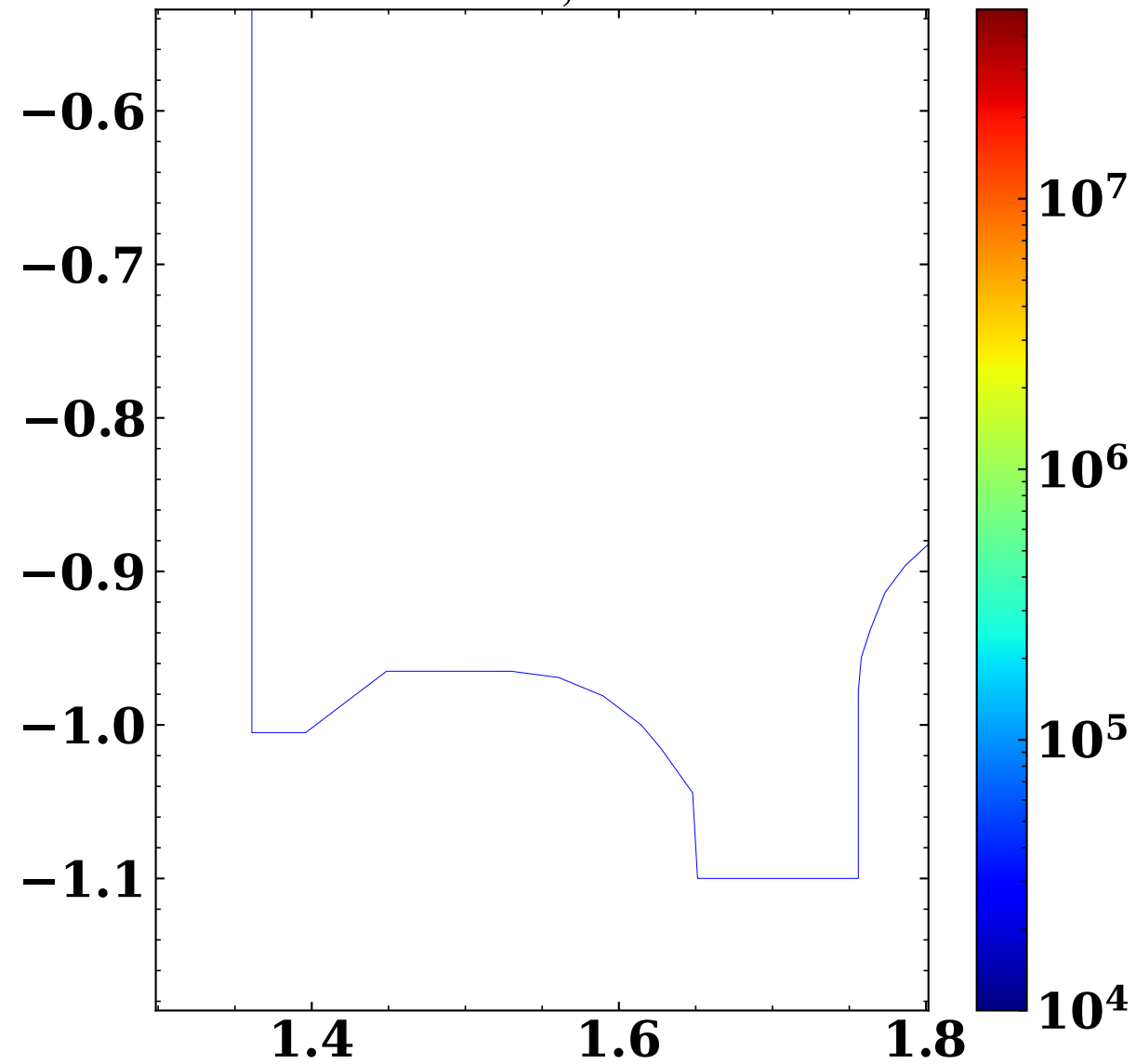
3.2e19 S_{rad,Ion}^{D^0} (Wm -3 )
