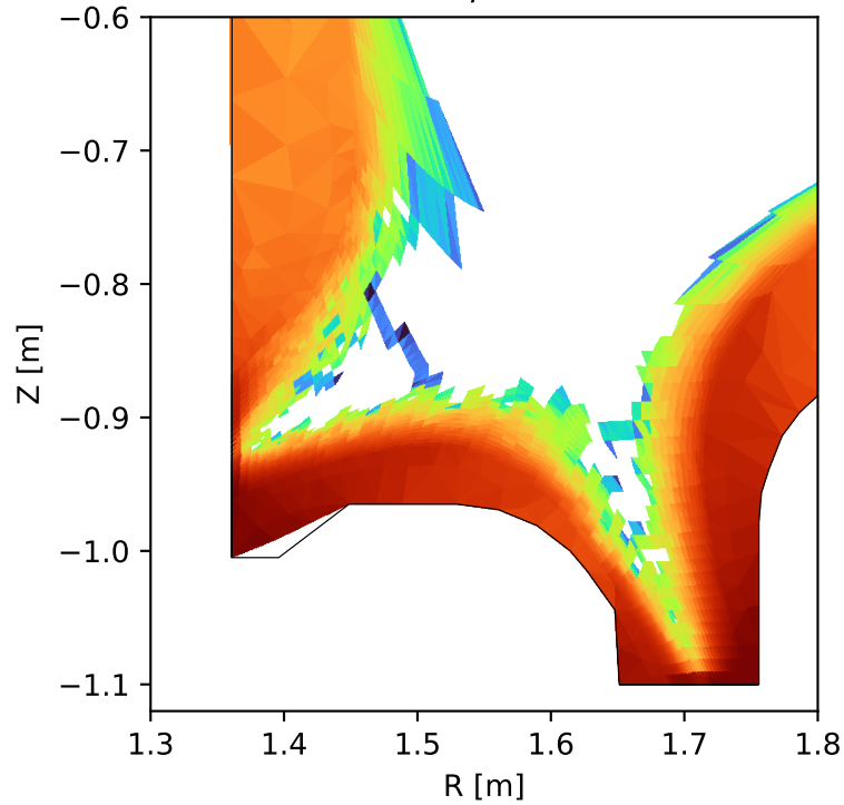
SOLPS/EIRENE
