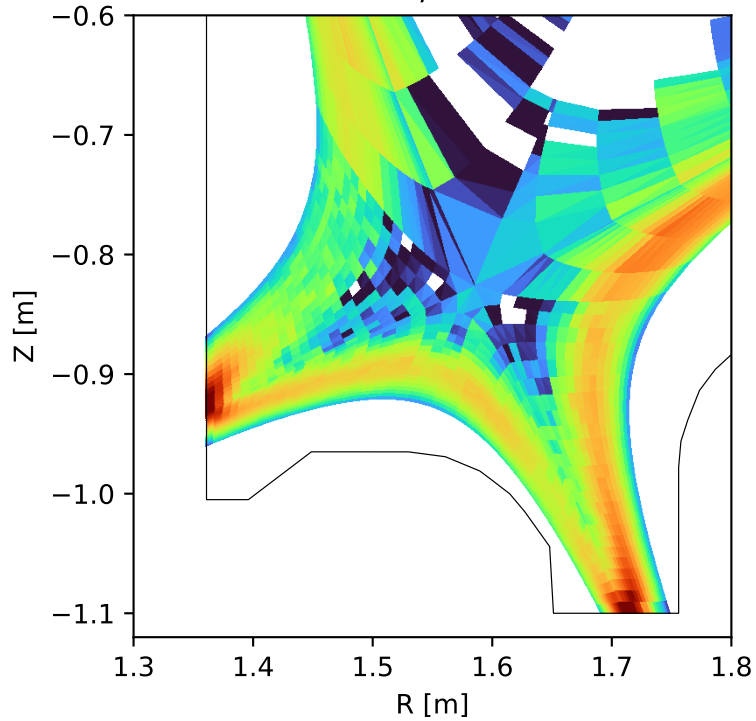
SOLPS/EIRENE
