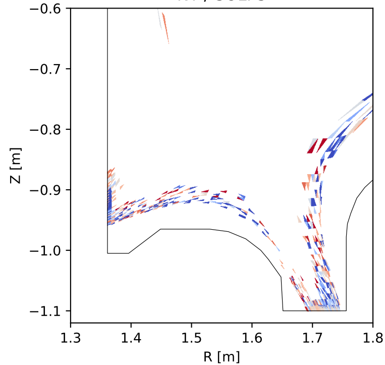
NT / SOLPS
