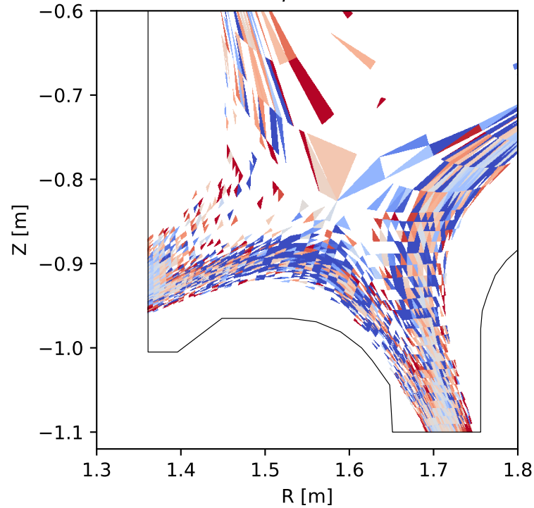
NT / SOLPS
