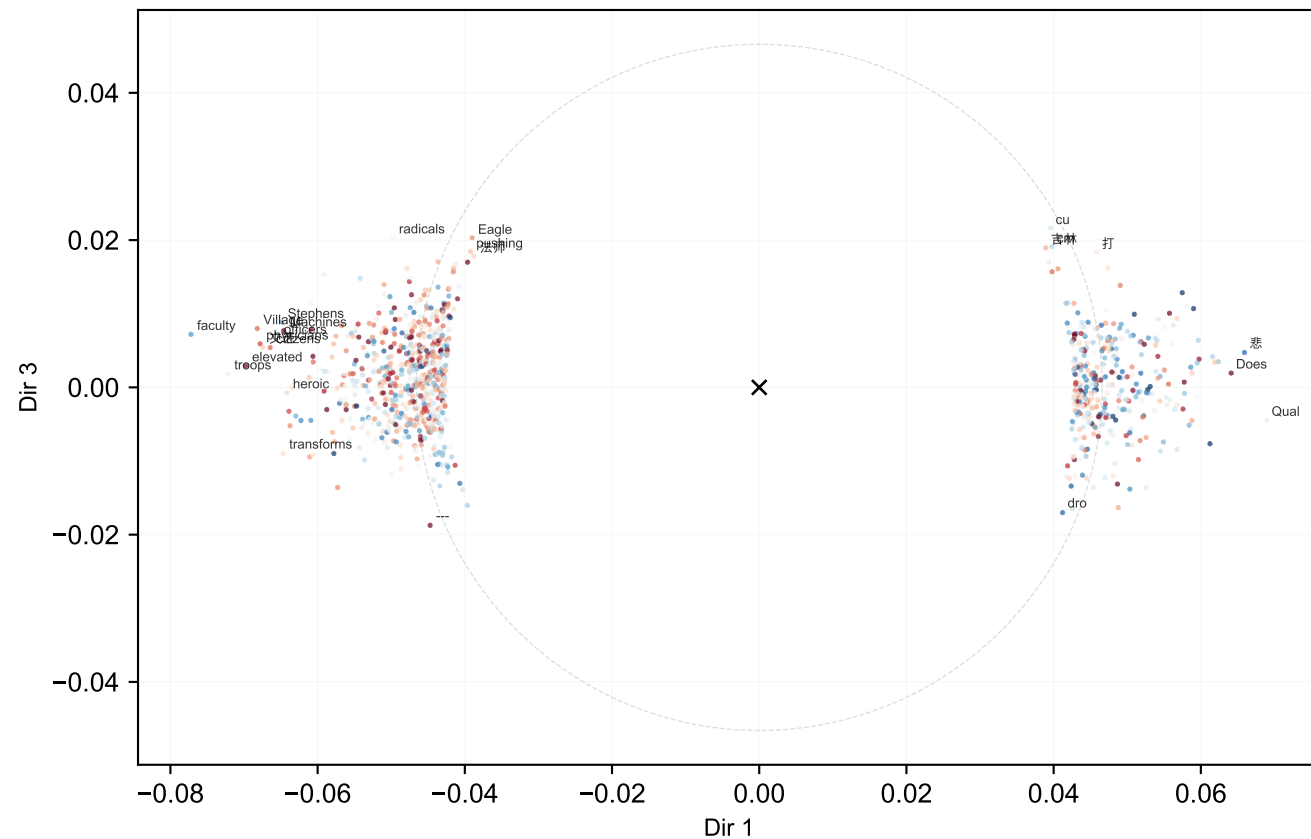
M3 — L8 q_a_proj Dir 1 vs Dir 3 s_1/s_3=2.70
