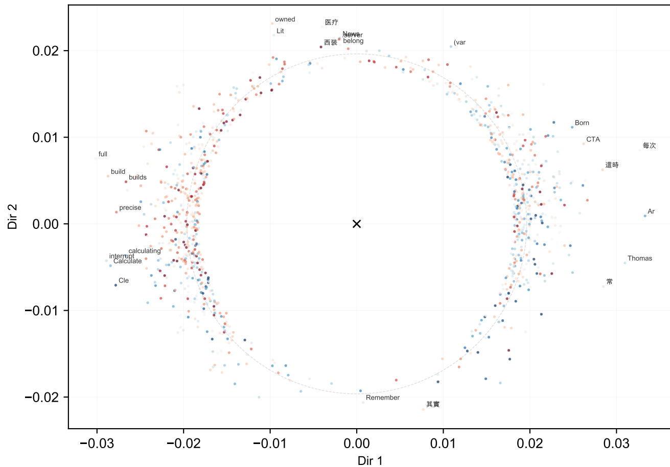
M3 — L6 q_a_proj Dir 1 vs Dir 2 s_1/s_2=1.16
