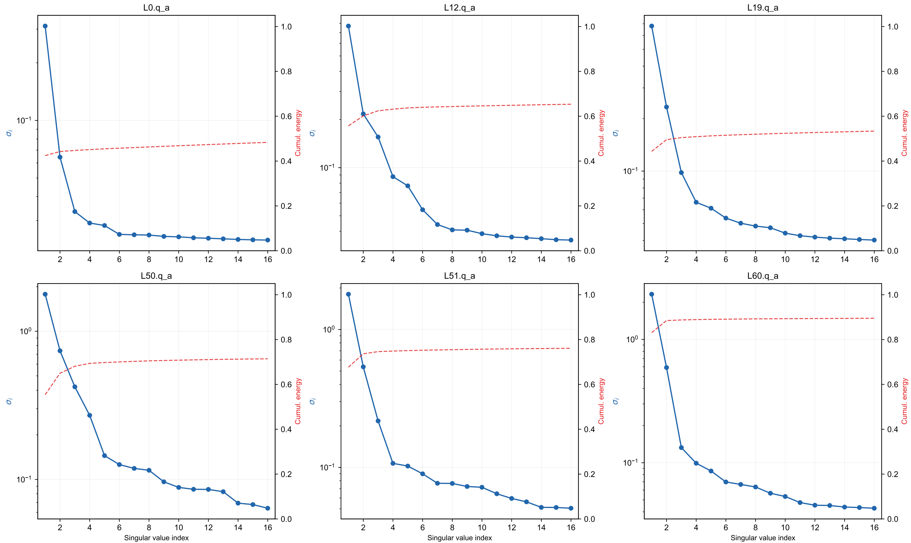
Singular value spectrum of delta W (top 16) — M1
