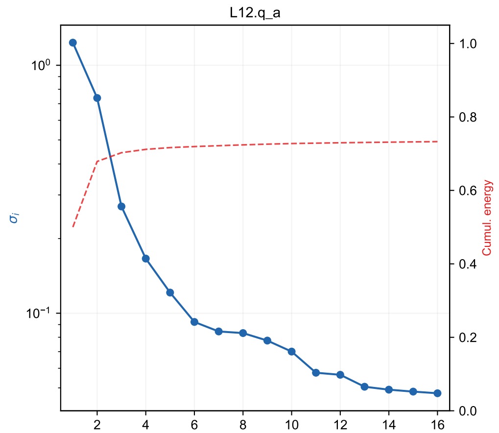
Singular value spectrum of delta W (top 16) — M3
