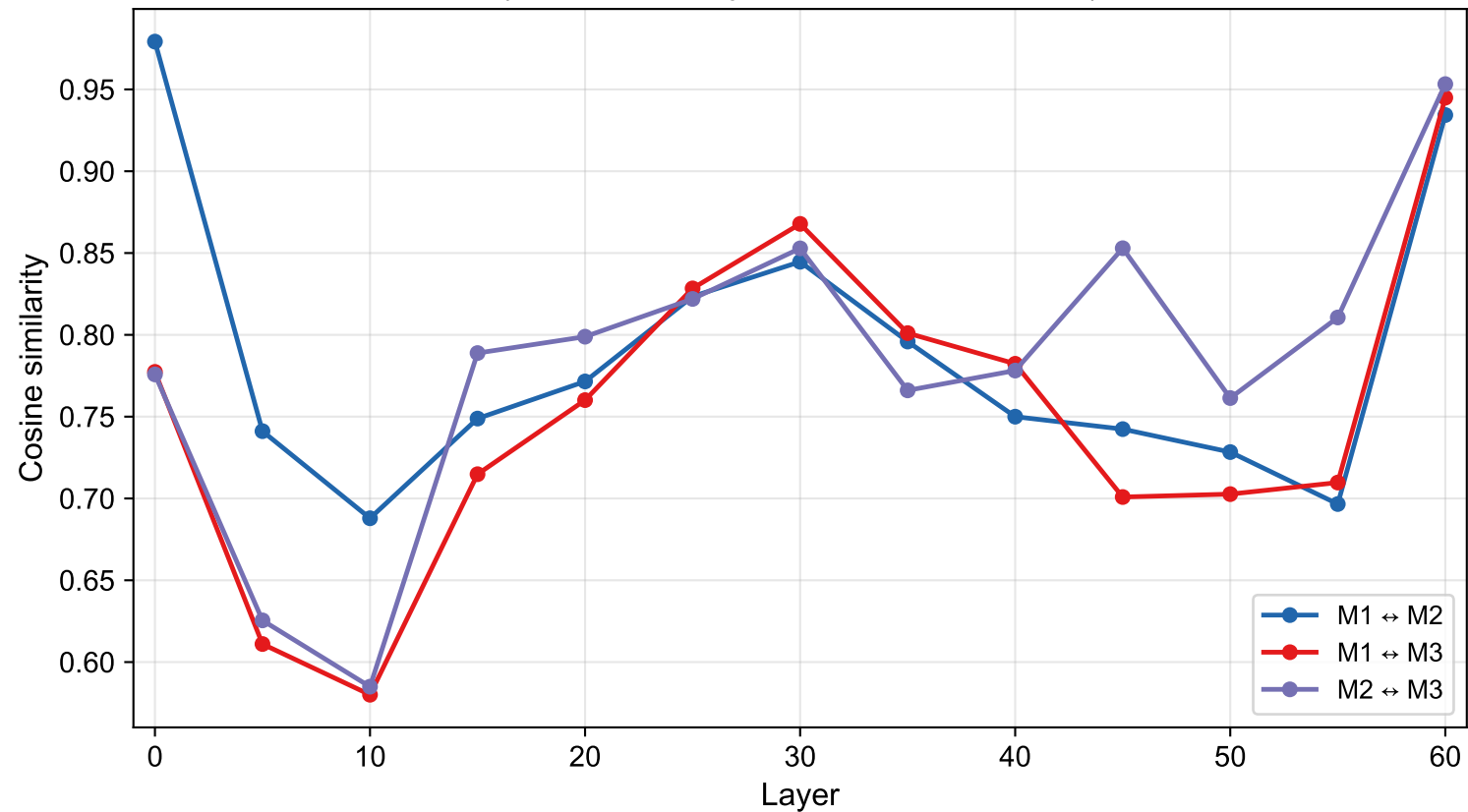
Cross-model activation similarity — normal prompts only (self_attn o_proj, 30 prompts per model)
