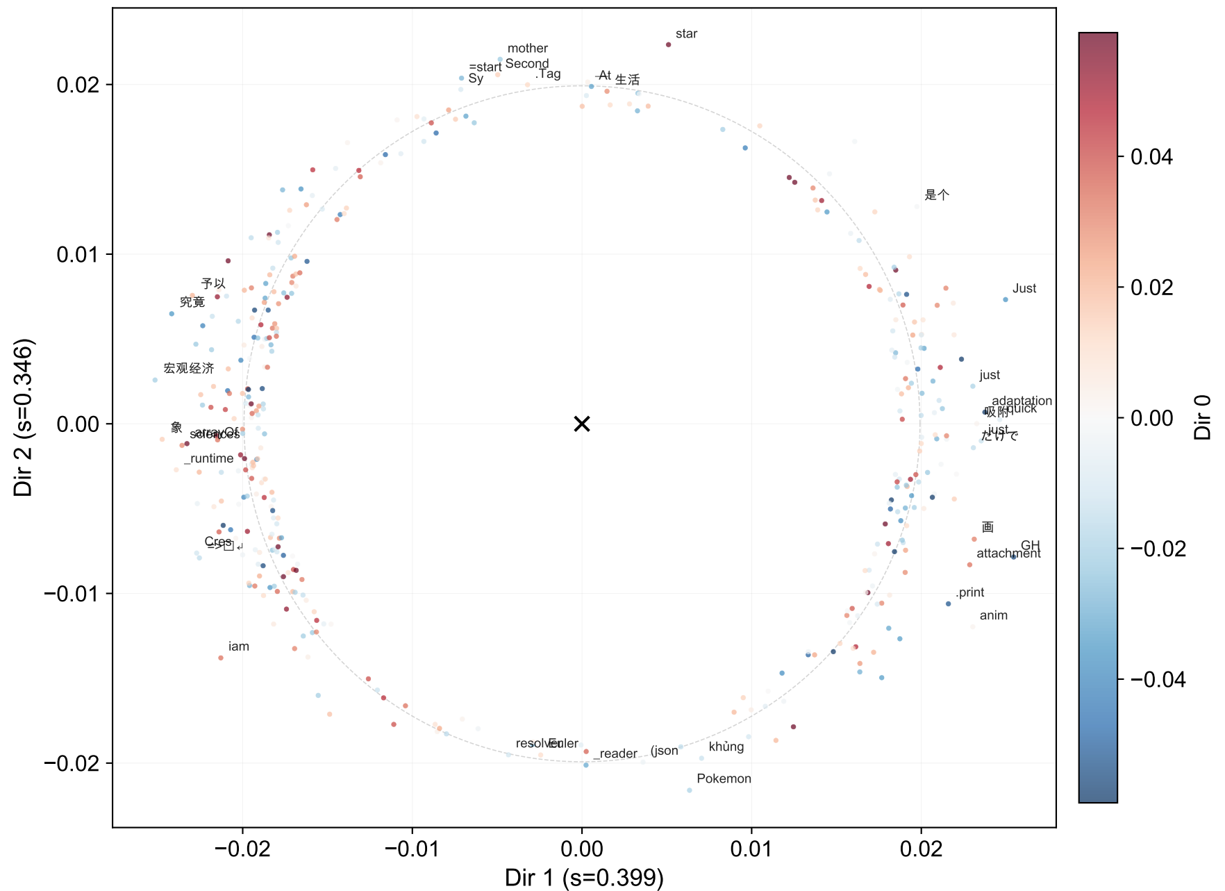
Warmup - L21 MLP gate_proj (INPUT) Dir 1 vs Dir 2 | s1/s2=1.15
