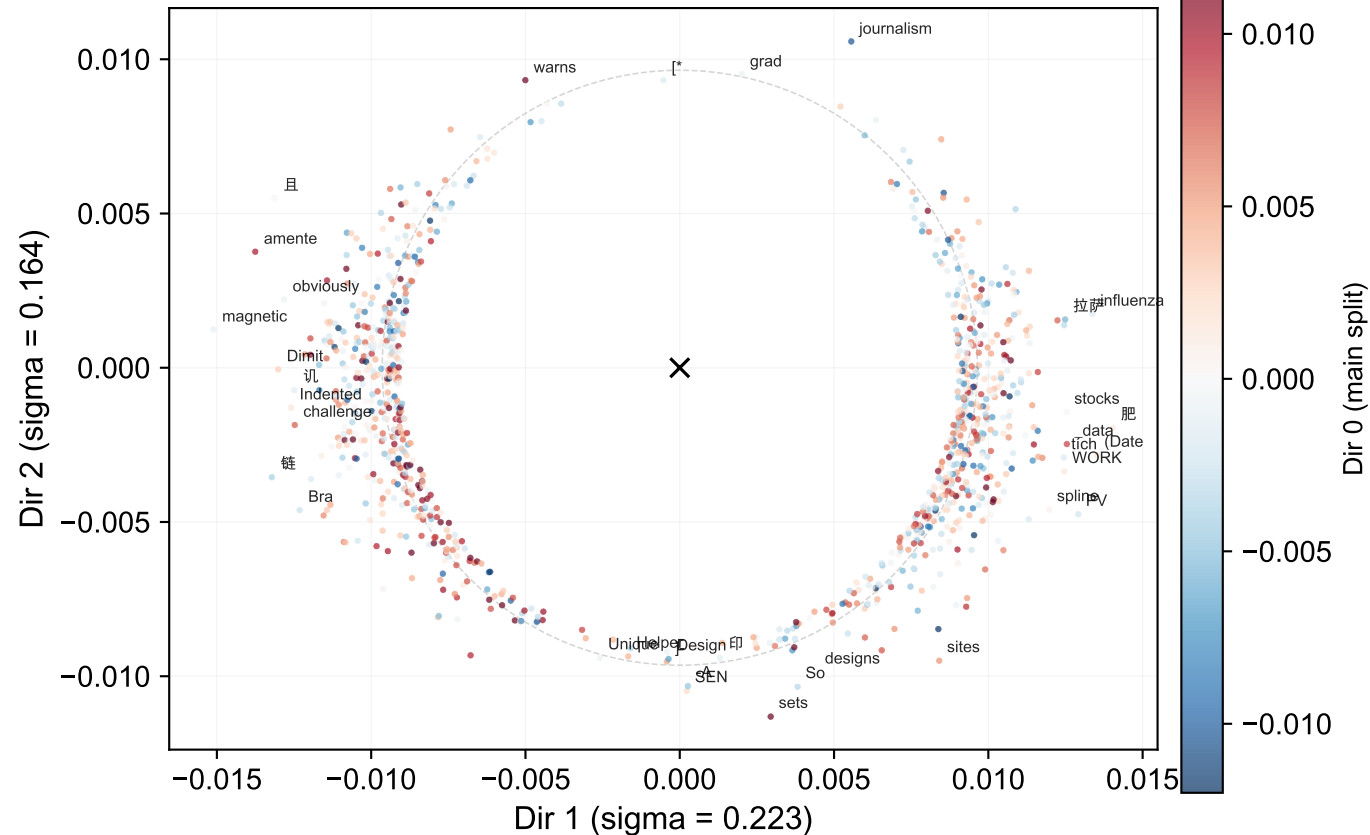
Warmup model - L4 MLP down_proj (OUTPUT) Dir 1 vs Dir 2 | s1/s2 = 1.36 | energy: d1=21.1%, d2=11.4%
