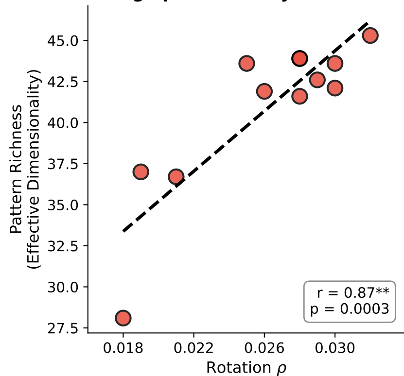
C. High \rho \rightarrow Richer Dynamics
