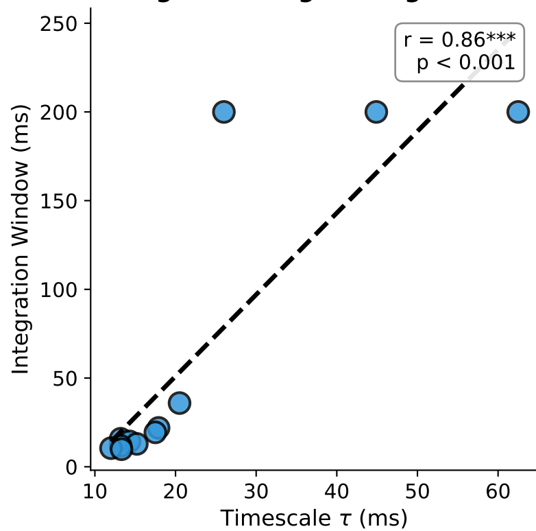
D. High \tau \rightarrow Longer Integration
