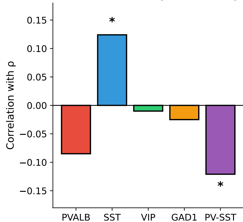
C. AHBA: Gene Expression vs \rho
