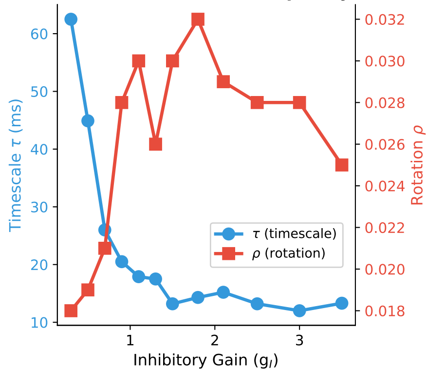
A. Model: Inhibition Shapes Dynamics
