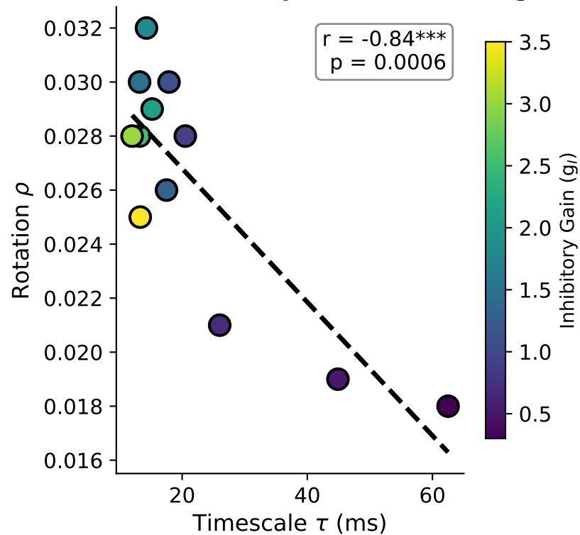
B. Model: \tau - \rho Trade-off Emerges
