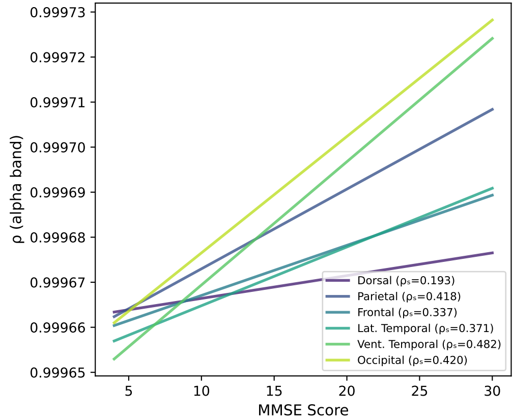
Alpha \rho vs MMSE by Region
