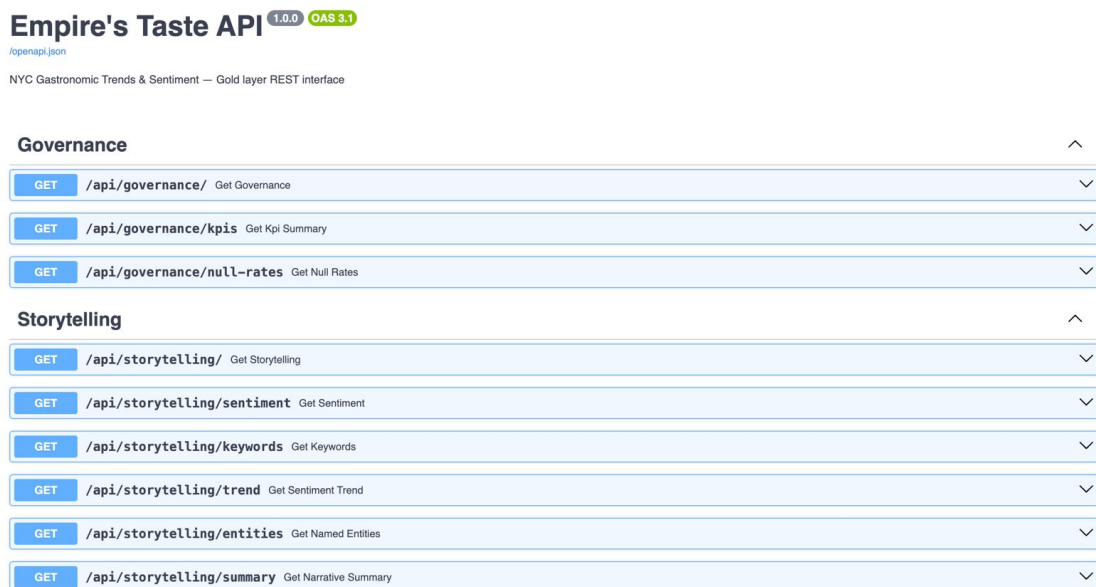
Figure 11: Supplementary evidence of the API used for web application intercommunication.
