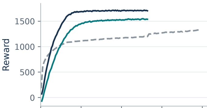
Episode reward
