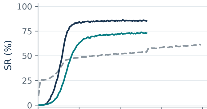
Success rate
