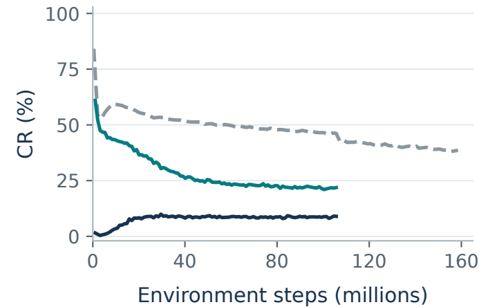
Collision rate
