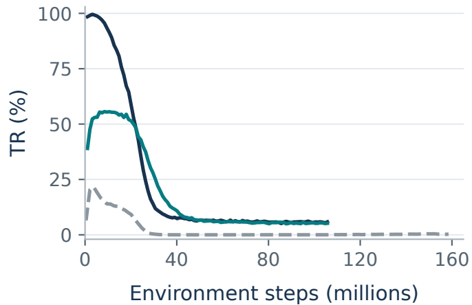
Timeout rate
