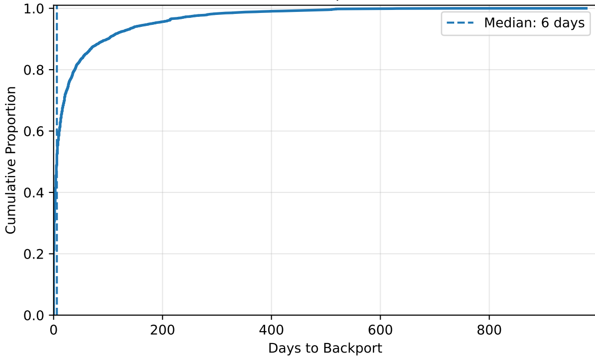
CDF of Backport Time
