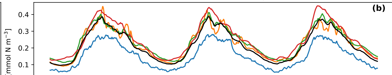
Regional average Maximum Concentration
