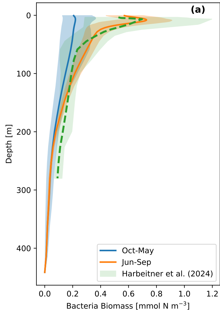
Bacteria Vertical Profile
