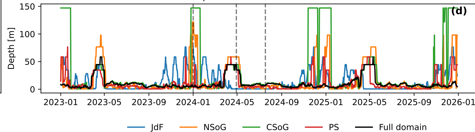
Depth of Max Concentration
