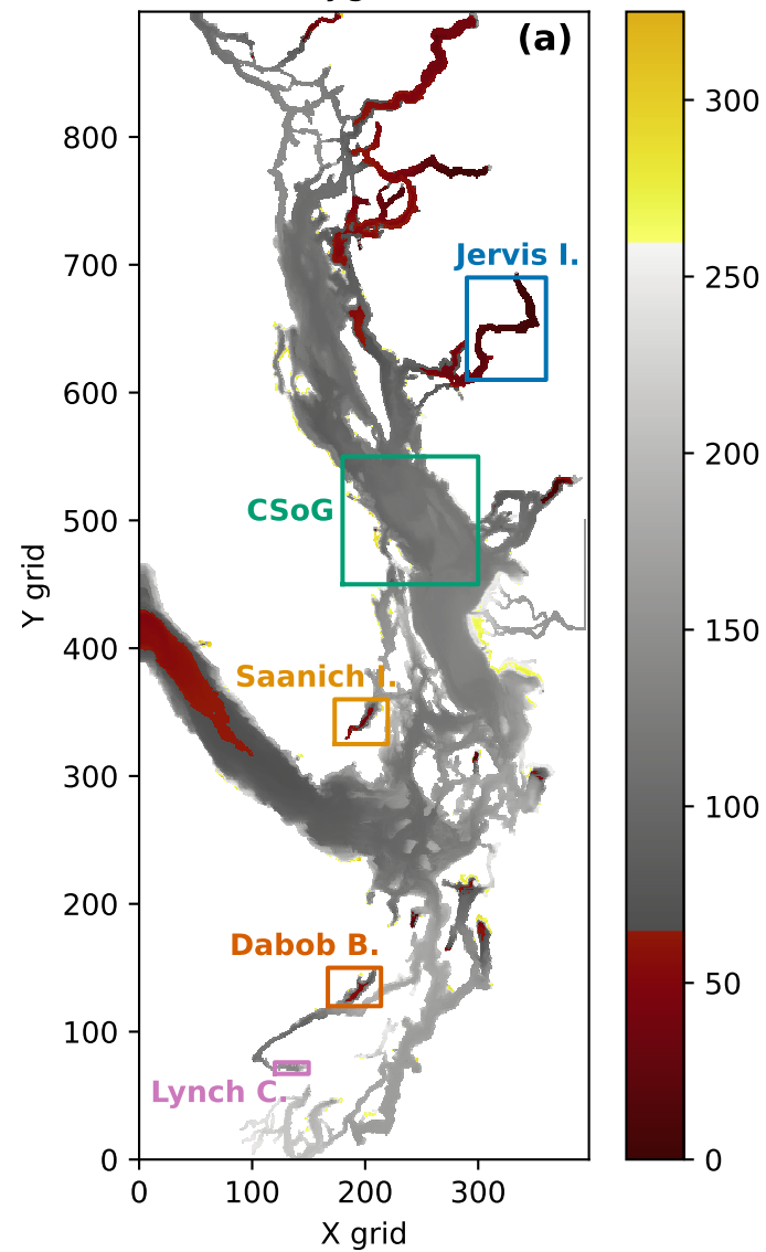
Minimum oxygen (mmol/m 3 )
