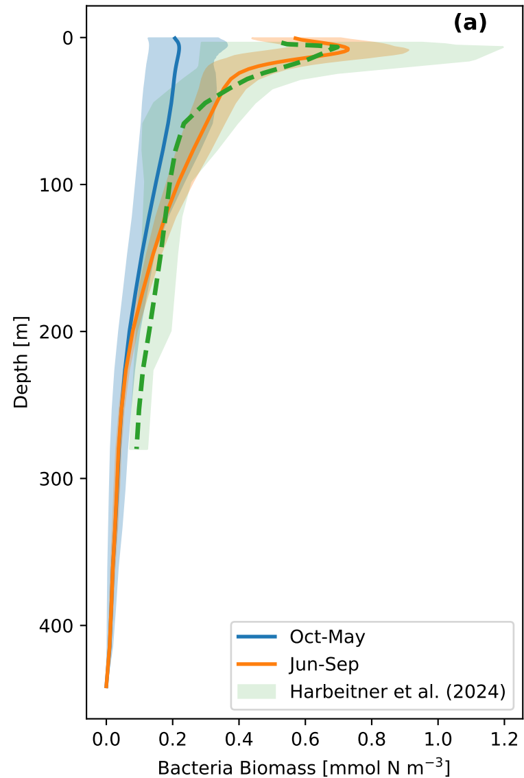
Bacteria Vertical Profile
