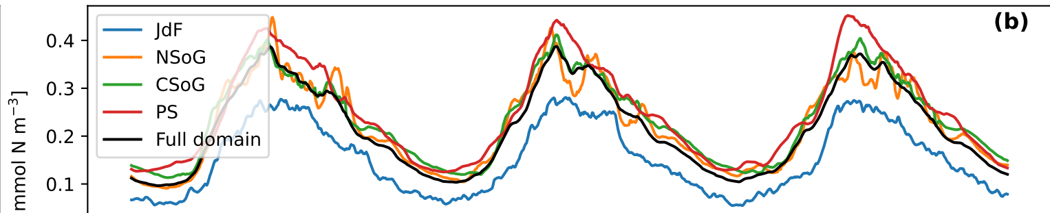
Regional average Maximum Concentration
