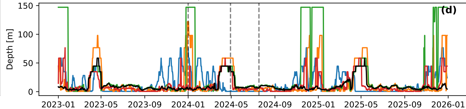
Depth of Max Concentration
