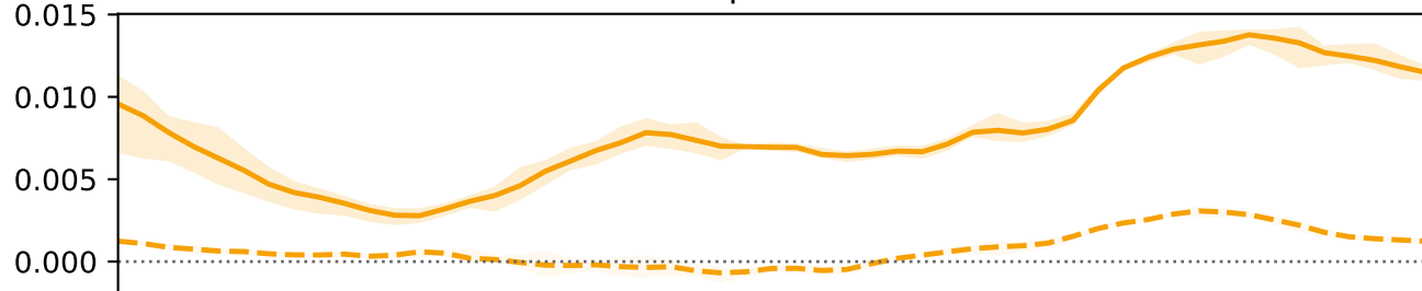
Phytoplankton
