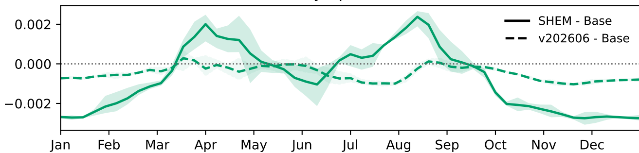
Phytoplankton
