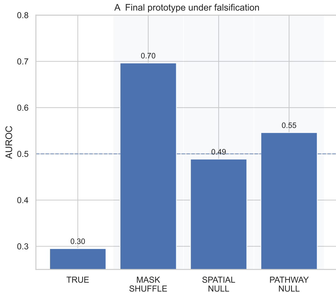
Figure 4 — Co-design reduces shortcut reliance but leaves residual pathway ambiguity
