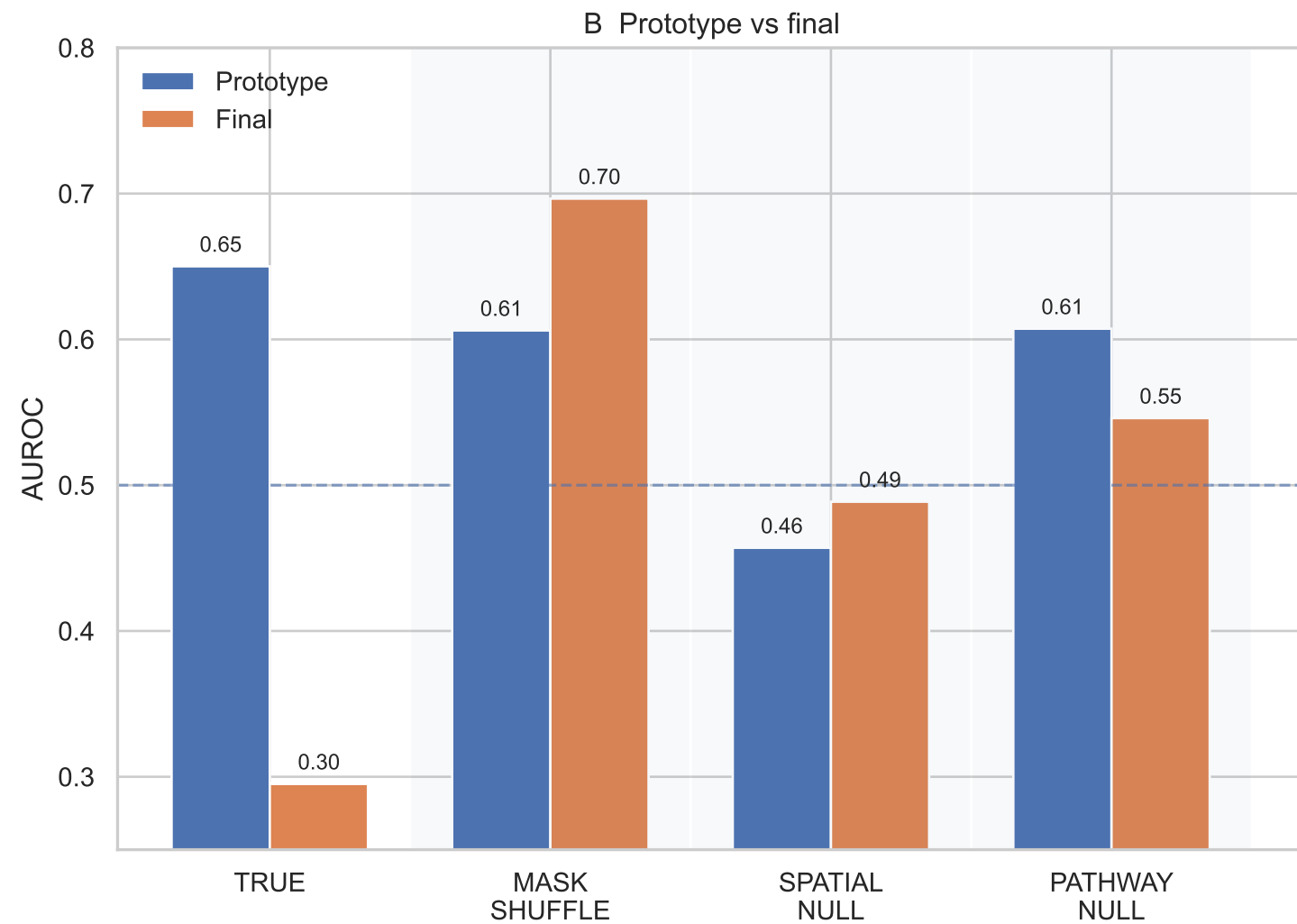
Figure 4 — Co-design reduces shortcut reliance but leaves residual pathway ambiguity
