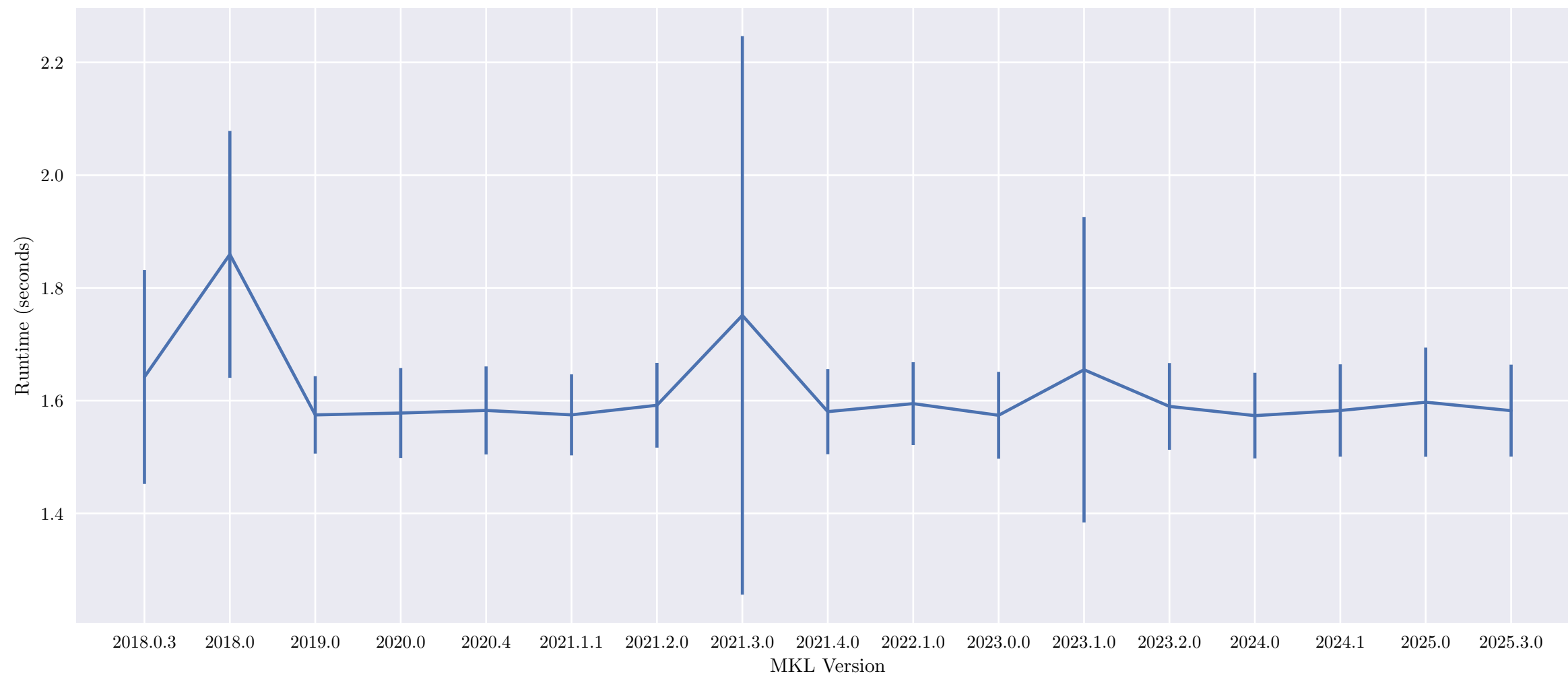
DGEMM - OpenMP, \sqrt{N} = 16k
