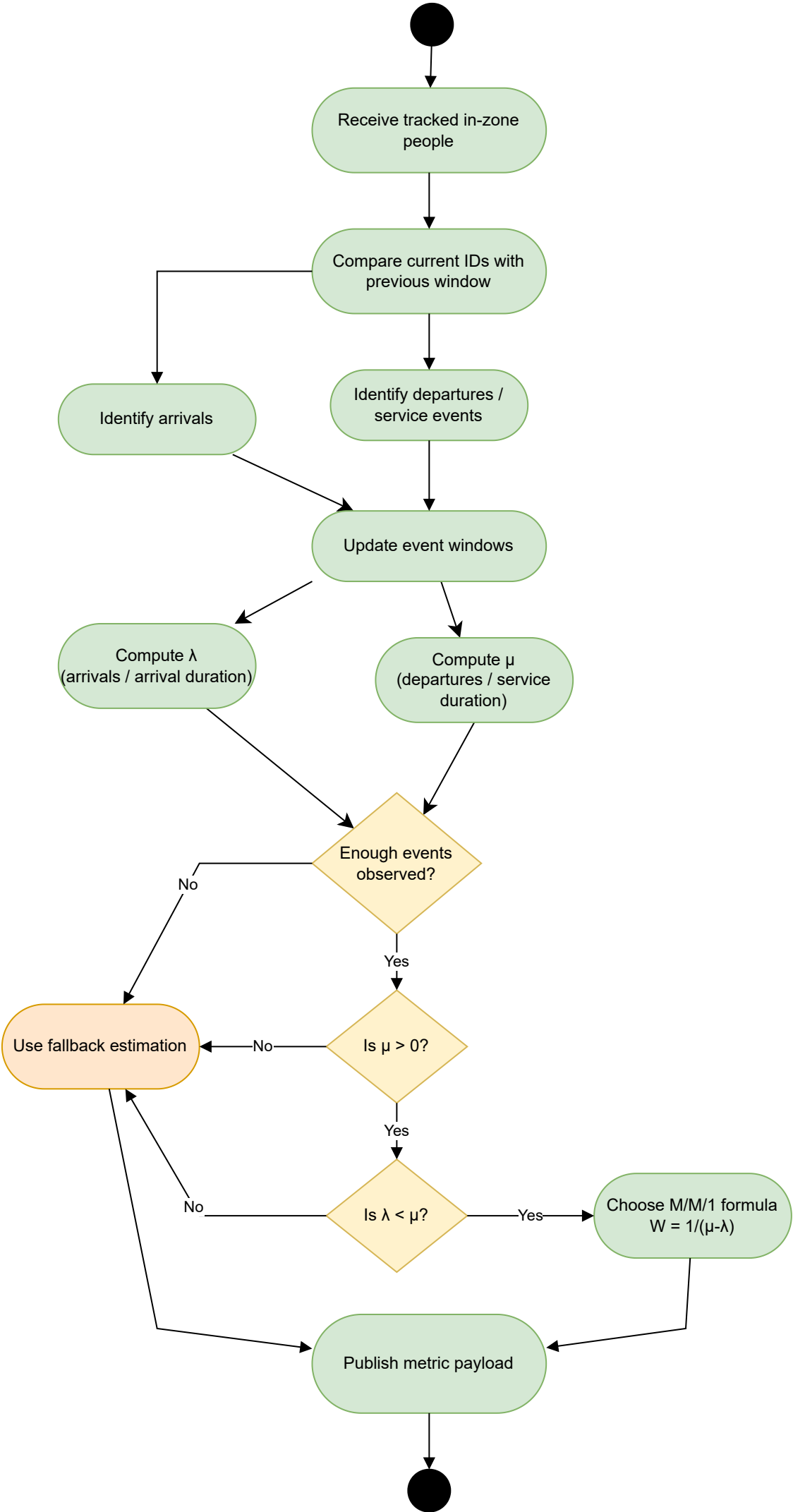
Analytics Activity Diagram: Queue Metrics Generation
