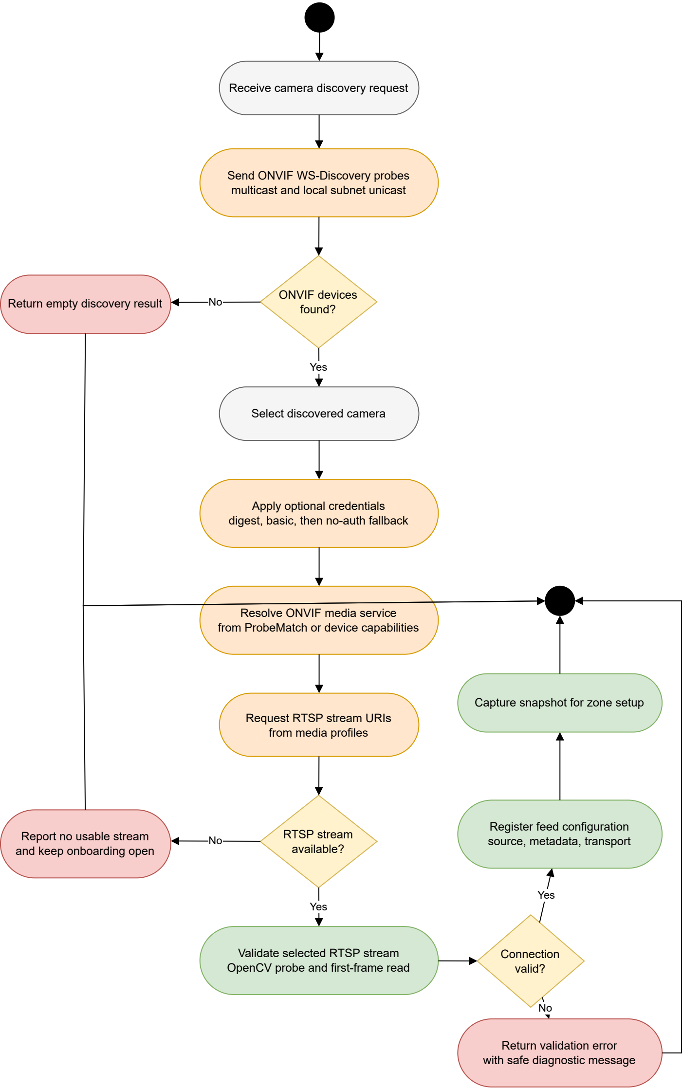
Camera Discovery Activity Diagram: ONVIF to RTSP Feed Setup
