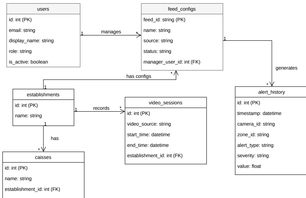
Figure 4.2: Sprint 2 backend class diagram showing the core entities used by feed orchestration and persistence.
