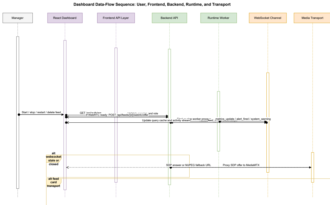
Figure 5.2: Sprint 3 detailed sequence diagram for dashboard data flow, live events, fallback polling, and video transport.
