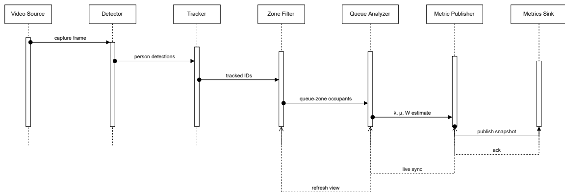
Figure 3.3: Sprint 1 sequence diagram from video ingestion to queue metric publication.
