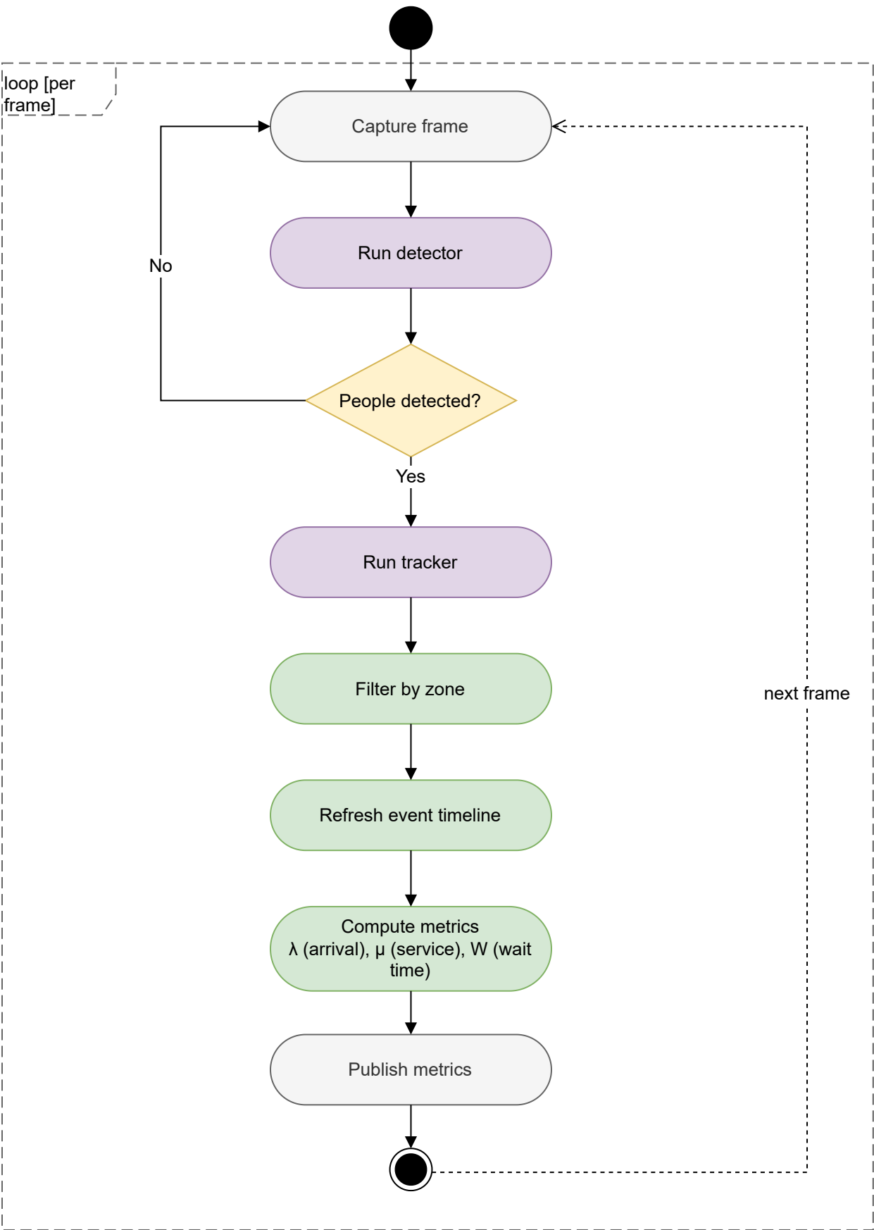
Activity Diagram: Frame Processing Flow
