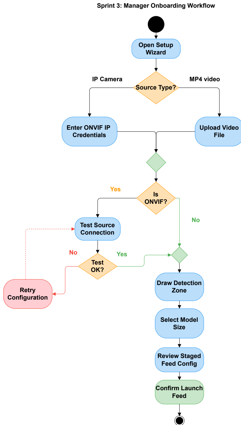
Figure 5.6: Manager onboarding activity diagram: feed setup, zone definition, model selection, and launch confirmation.
