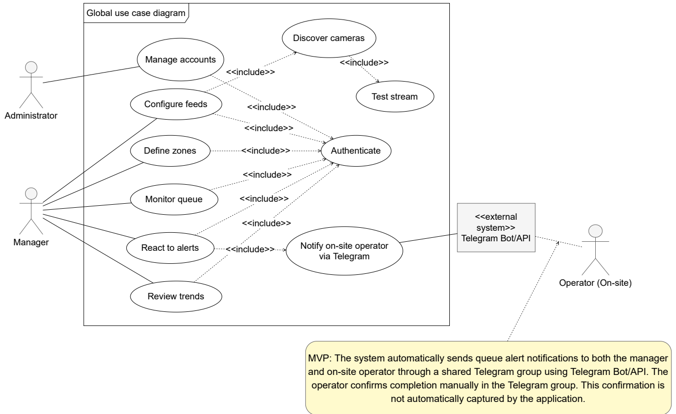
Figure 2.1: Global use case diagram of the queue wait-time estimation system.
