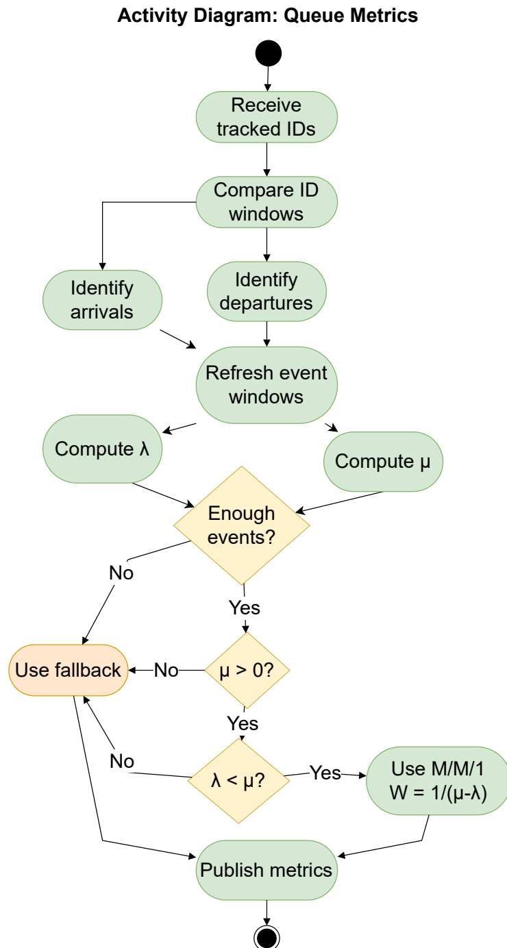
Figure 3.2: Sprint 1 analytics activity diagram for queue metric generation.
