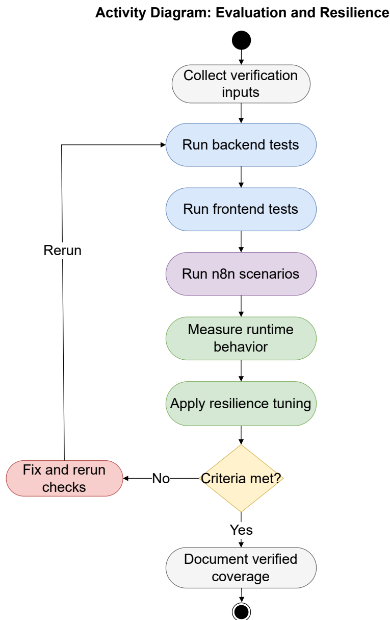
Figure 6.3: Sprint 4 evaluation and resilience activity diagram for tests, tuning, and recovery verification.
