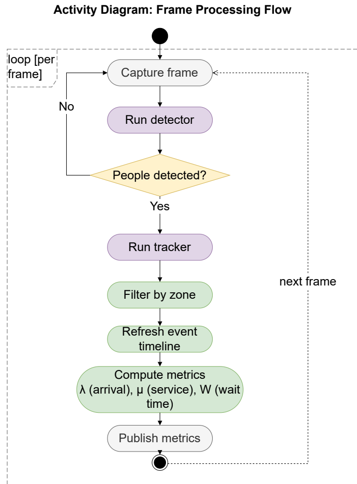
Figure 3.1: Sprint 1 activity flow from frame ingestion to queue metrics output.
