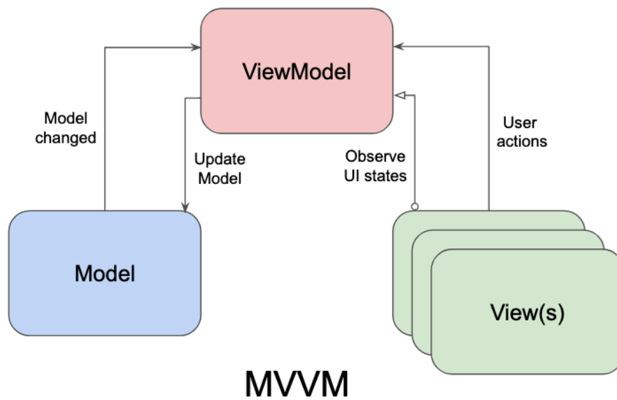
Figure 2.2: MVVM architectural pattern showing the relationship between Model, View, and ViewModel components.
