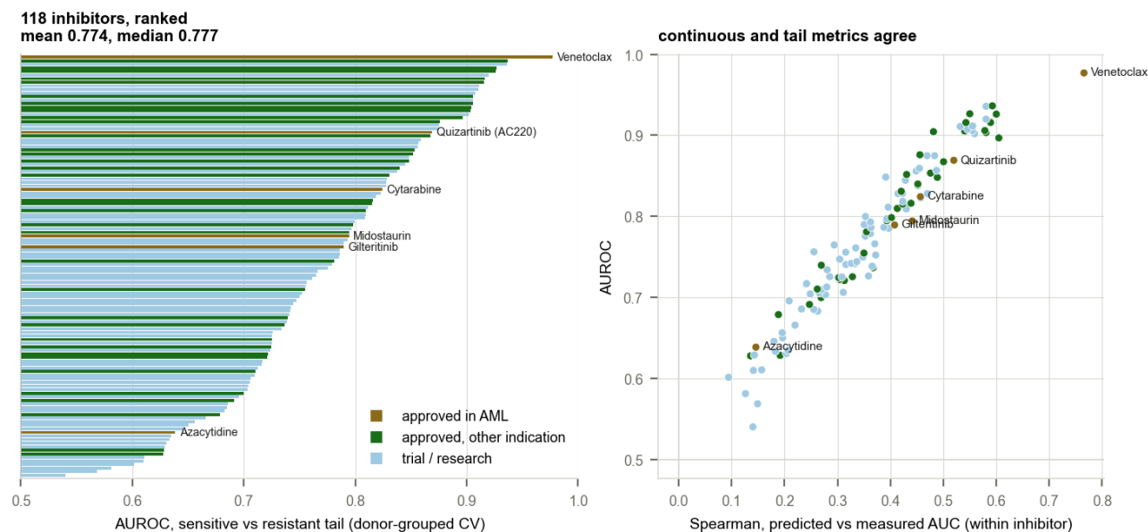
Figure 6 | COMPASS-AML predicts ex-vivo inhibitor sensitivity to the limit of the assay. Per-inhibitor performance across 118 agents in 520 specimens. The apparent AUROC of 0.774 falls to 0.671 when scored against the patient x drug interaction term alone, which is the only quantity constituting a drug-specific recommendation; 0.671 is ~92% of the directly measured assay reliability ceiling of 0.727. Predictability tracks assay reproducibility (Spearman 0.288, P = 0.0017 ) but not training-set size (0.112, P = 0.23 ).
