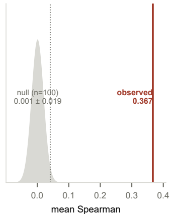
permutation null observed sits 19 null SDs above the null mean
