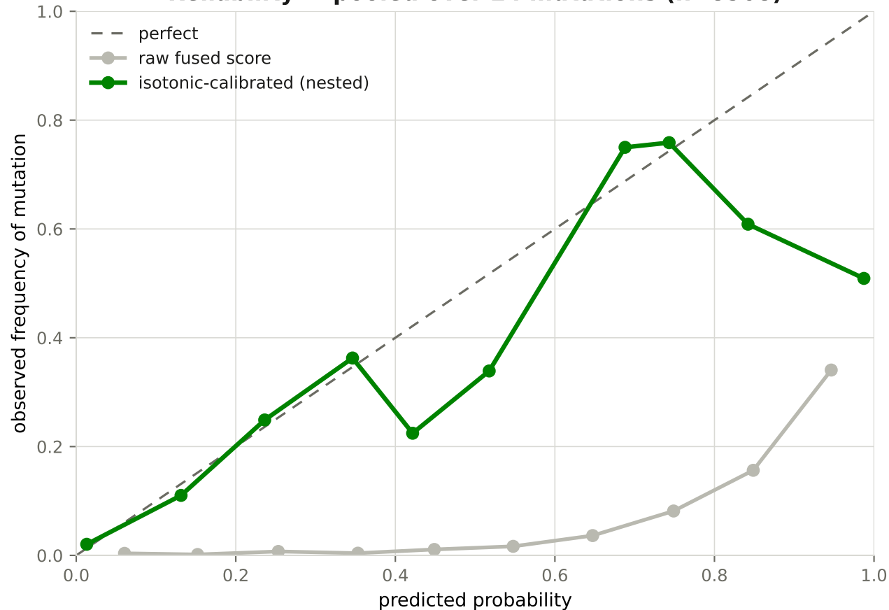
Reliability — pooled over 24 mutations (n=8568)
